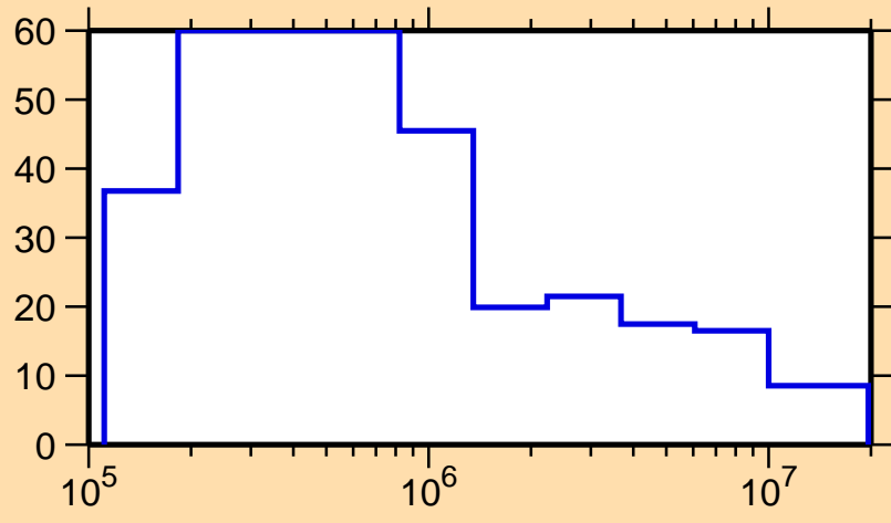
\Delta\sigma/\sigma vs. E for ^{205}\text{Au}(n, \text{tot.})
