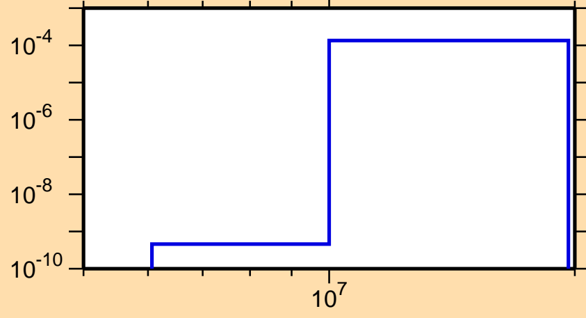
\sigma vs. E for ^{205}\text{Au}(n,p)
