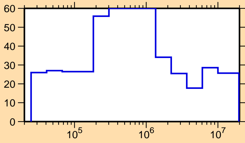
\Delta\sigma/\sigma vs. E for ^{205}\text{Au}(n,\text{el.})
