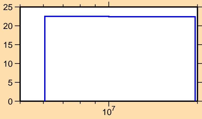
\Delta\sigma/\sigma vs. E for ^{205}\text{Au}(n,\text{nonel.})
