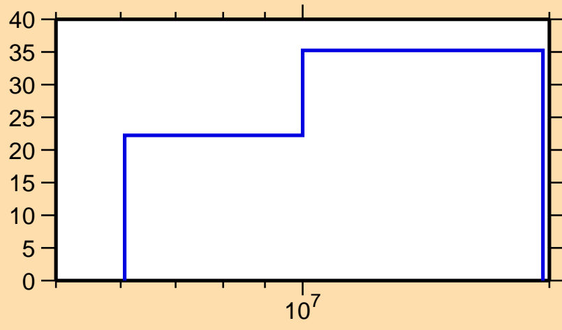
\Delta\sigma/\sigma vs. E for ^{205}\text{Au}(n,2n)
