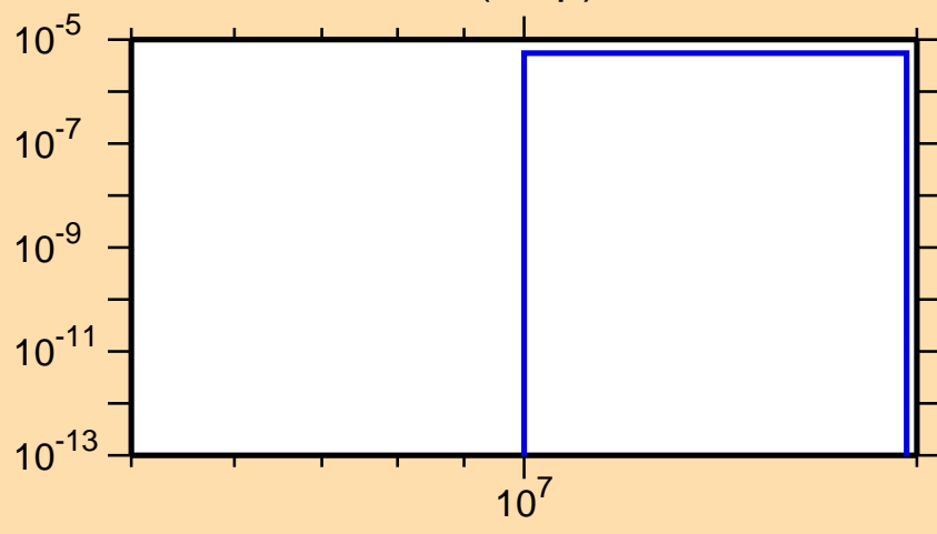
\sigma vs. E for ^{205}\text{Au}(n,np)
