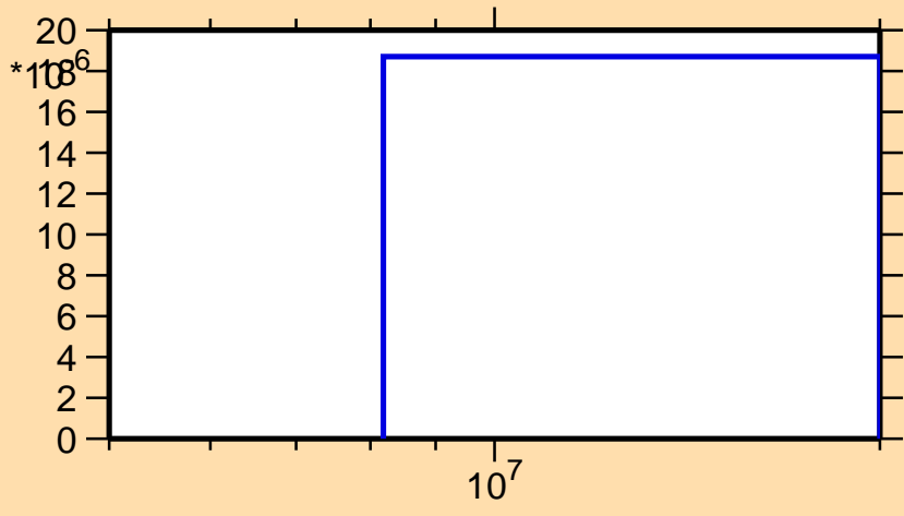
\sigma vs. E for ^{205}\text{Au}(n,d)
