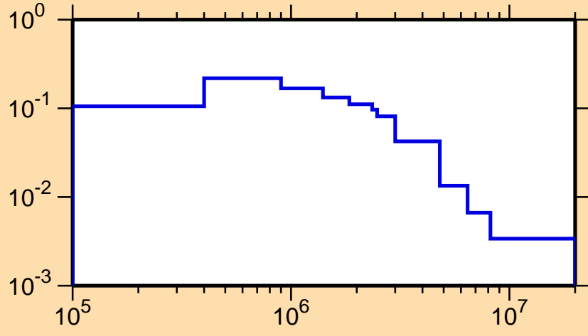
\sigma vs. E for ^{205}\text{Au}(n,n_1)
