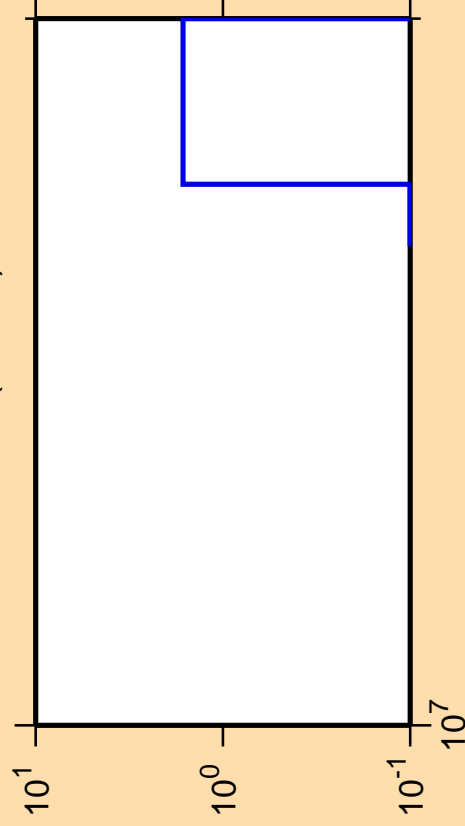
\Delta\sigma/\sigma vs. E for ^{206}\text{Au}(n,3n\alpha)
