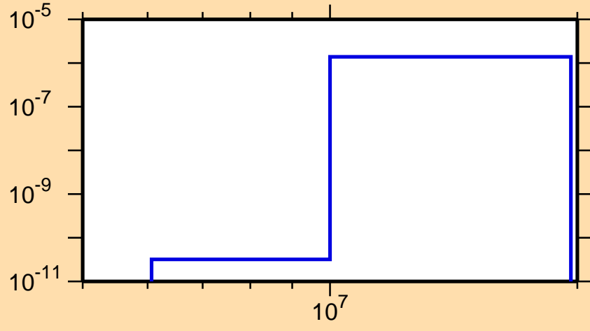
\sigma vs. E for ^{206}\text{Au}(n,n\alpha)
