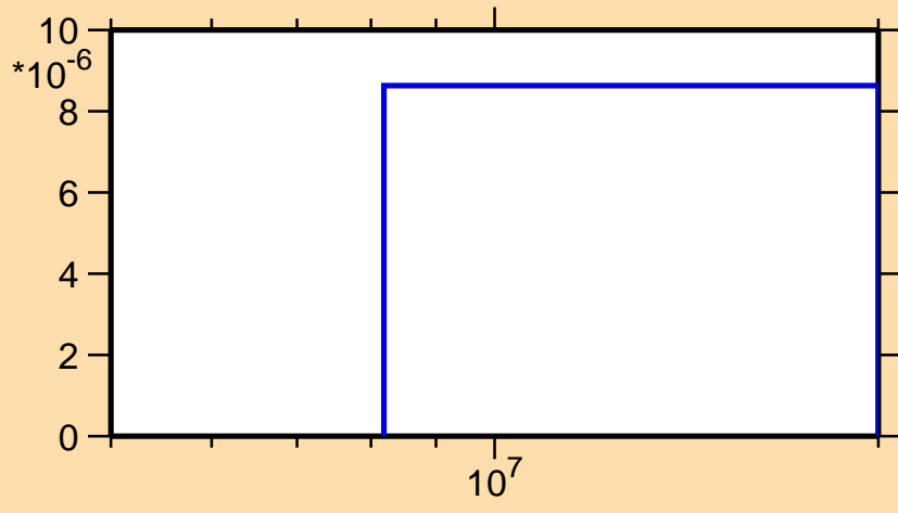
\sigma vs. E for ^{206}\text{Au}(n,np)
