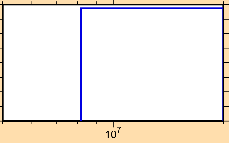
\sigma vs. E for ^{206}\text{Au}(n,d)
