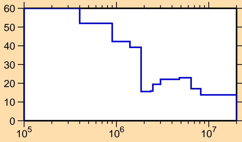
\Delta\sigma/\sigma vs. E for ^{206}\text{Au}(n,n\text{cont.})
