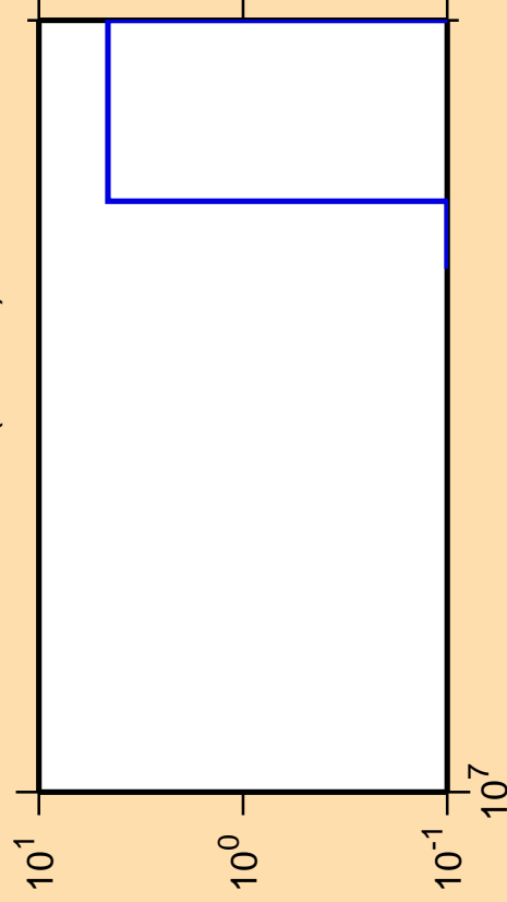
\Delta\sigma/\sigma vs. E for ^{207}\text{Au} (mt 42)
