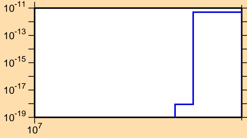
\sigma vs. E for ^{207}\text{Au} (mt 42)
