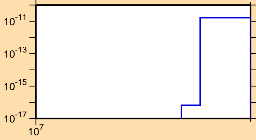
\sigma vs. E for ^{207}\text{Au} (mt 11)
