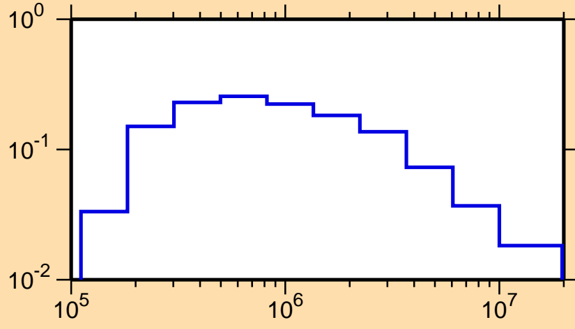
\sigma vs. E for ^{207}\text{Au}(n,n_1)
