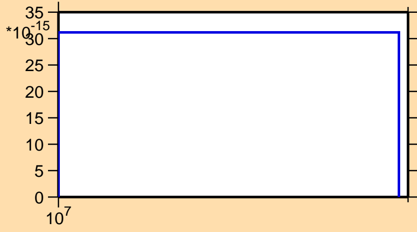
\sigma vs. E for ^{207}\text{Au} (mt 42)
