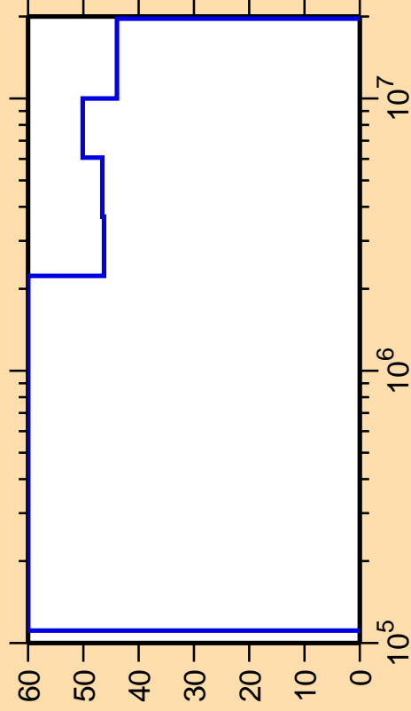
\Delta\sigma/\sigma vs. E for ^{207}\text{Au}(n,n_1)
