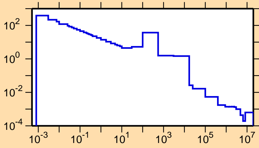
\sigma vs. E for ^{207}\text{Au}(n,\gamma)
