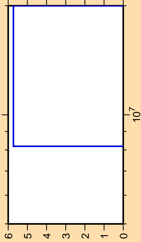
\Delta\sigma/\sigma vs. E for ^{207}\text{Au}(n,3n)
