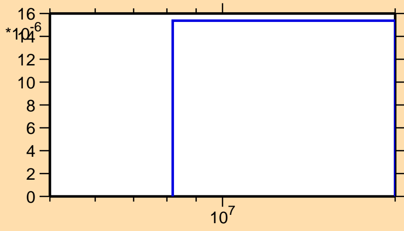
\sigma vs. E for ^{207}\text{Au}(n,t)
