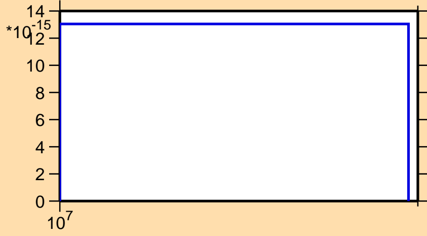
\sigma vs. E for ^{208}\text{Au} (mt 42)
