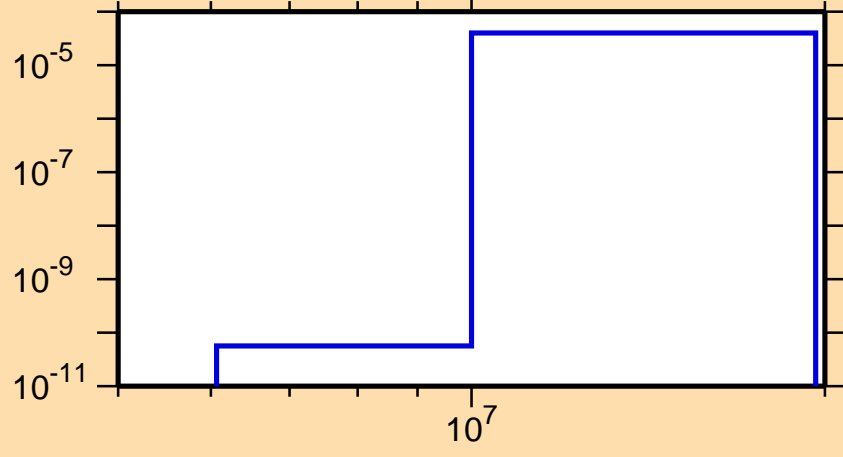
\sigma vs. E for ^{208}\text{Au}(n,t)
