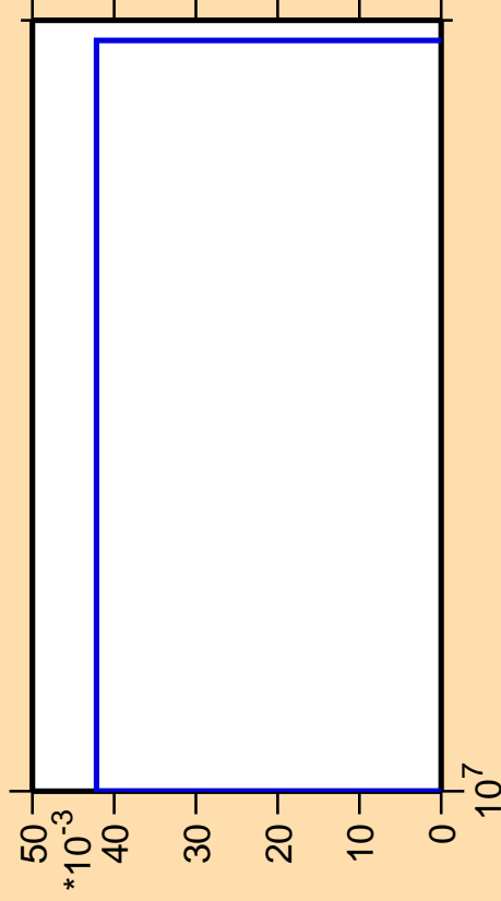
\Delta\sigma/\sigma vs. E for ^{208}\text{Au} (mt 42)
