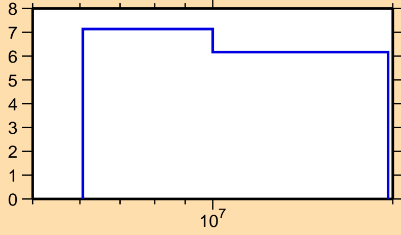
\Delta\sigma/\sigma vs. E for ^{208}\text{Au}(n,\text{nonel.})
