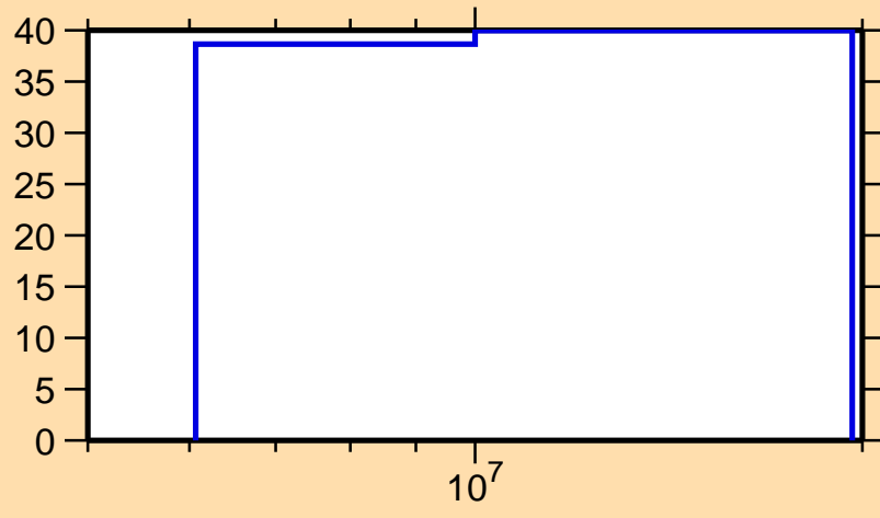
\Delta\sigma/\sigma vs. E for ^{208}\text{Au}(n,n\text{cont.})
