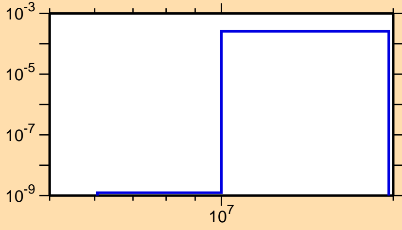
\sigma vs. E for ^{208}\text{Au}(n,p)
