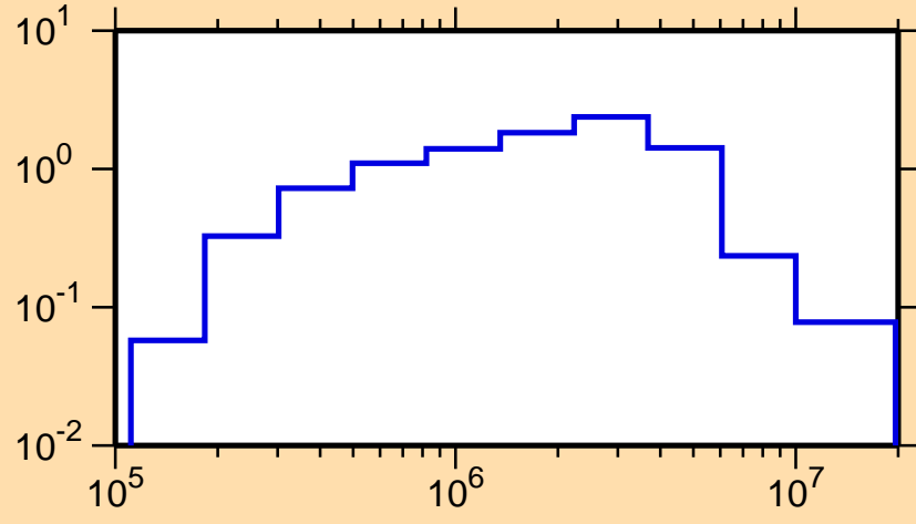
\sigma vs. E for ^{208}\text{Au}(n,n\text{cont.})
