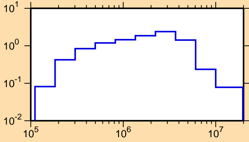
\sigma vs. E for ^{208}\text{Au}(n,\text{inel.})
