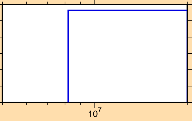
\sigma vs. E for ^{208}\text{Au}(n,nd)
