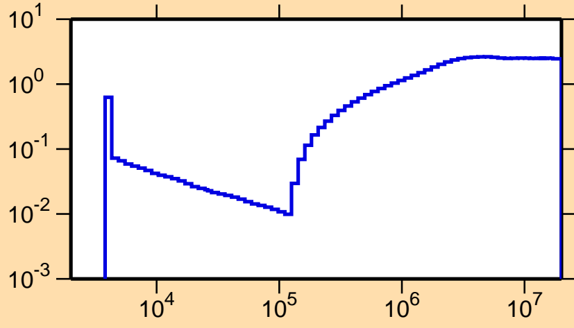
\sigma vs. E for ^{209}\text{Au}(n,\text{nonel.})
