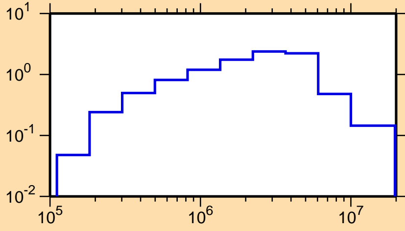
\sigma vs. E for ^{209}\text{Au}(n,\text{inel.})
