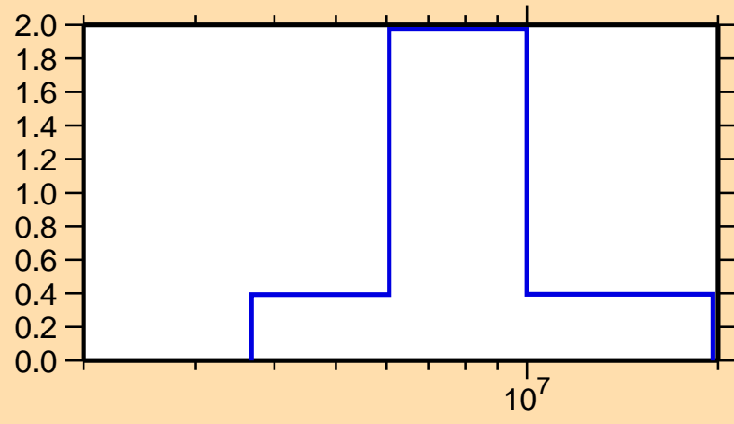
\sigma vs. E for ^{209}\text{Au}(n,2n)
