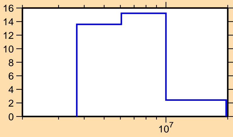
\Delta\sigma/\sigma vs. E for ^{209}\text{Au}(n,\text{tot.})
