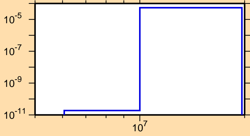
\sigma vs. E for ^{209}\text{Au}(n,p)
