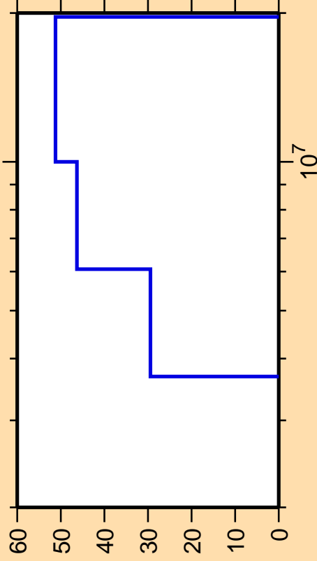
\Delta\sigma/\sigma vs. E for ^{209}\text{Au}(n,n\text{cont.})
