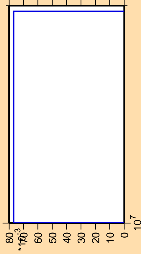
\Delta\sigma/\sigma vs. E for ^{209}\text{Au} (mt 42)
