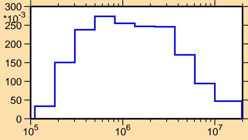
\sigma vs. E for ^{209}\text{Au}(n,n_1)
