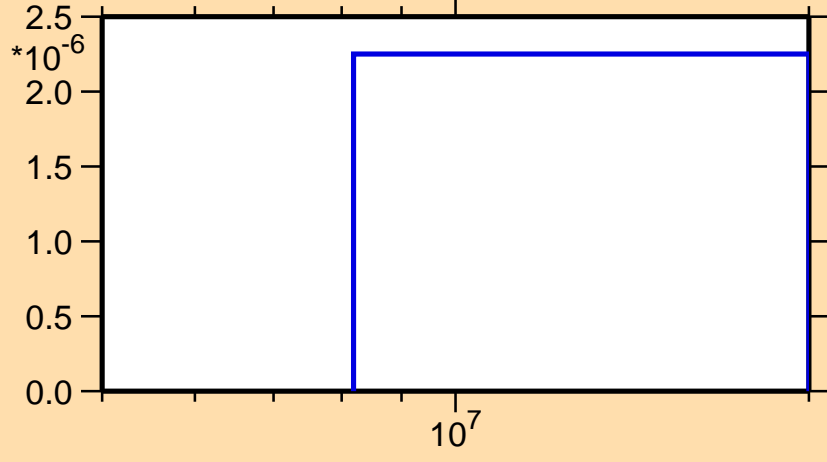
\sigma vs. E for ^{209}\text{Au}(n,np)
