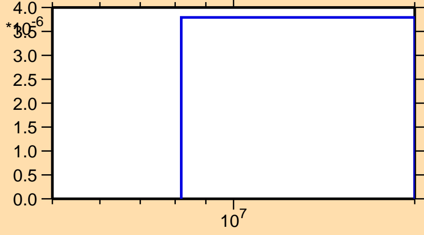
\sigma vs. E for ^{209}\text{Au}(n,d)
