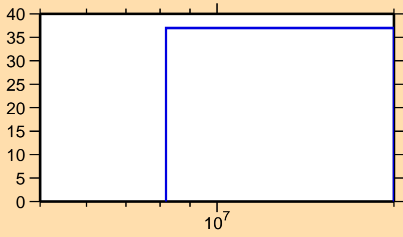
\Delta\sigma/\sigma vs. E for ^{209}\text{Au}(n,2n)
