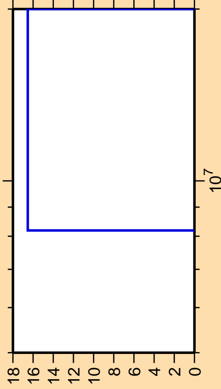
\Delta\sigma/\sigma vs. E for ^{209}\text{Au}(\text{mt } 11)
