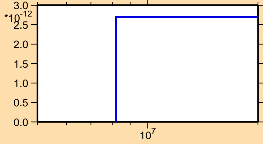
\sigma vs. E for ^{209}\text{Au}(\text{mt } 11)
