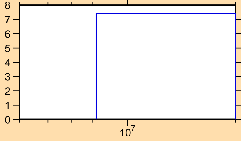
\Delta\sigma/\sigma vs. E for ^{209}\text{Au}(n,el.)
