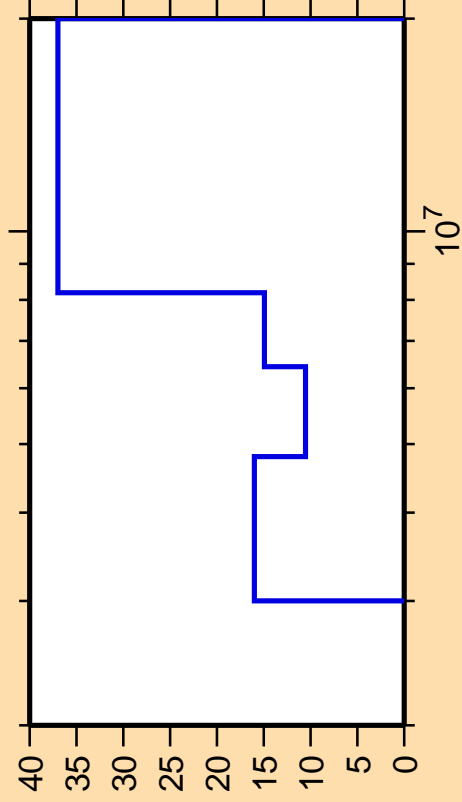
\Delta\sigma/\sigma vs. E for ^{209}\text{Au}(n,2n)
