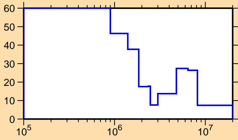
\Delta\sigma/\sigma vs. E for ^{209}\text{Au}(n, el.)
