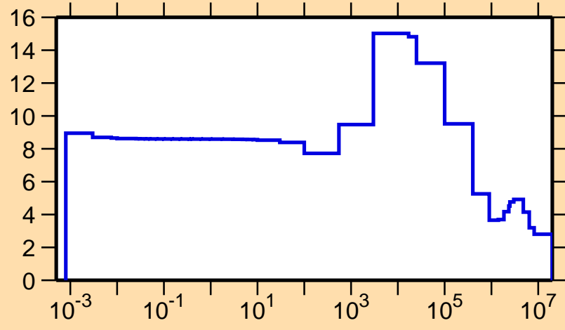
\sigma vs. E for ^{209}\text{Au}(n,\text{el.})
