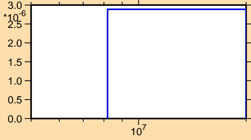
\sigma vs. E for ^{209}\text{Au}(n,nt)
