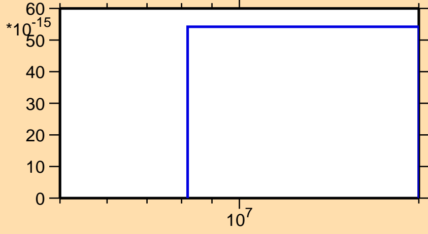
\sigma vs. E for ^{209}\text{Au}(\text{mt } 42)
