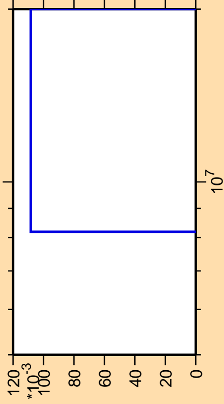
\Delta\sigma/\sigma vs. E for ^{209}\text{Au}(\text{mt } 42)
