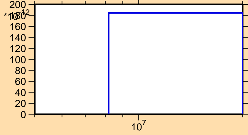
\sigma vs. E for ^{209}\text{Au}(n,2np)
