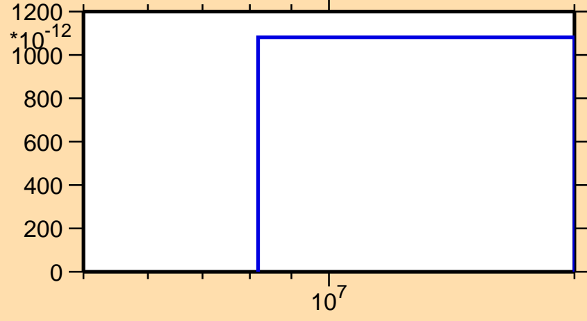
\sigma vs. E for ^{209}\text{Au}(n,3n\alpha)
