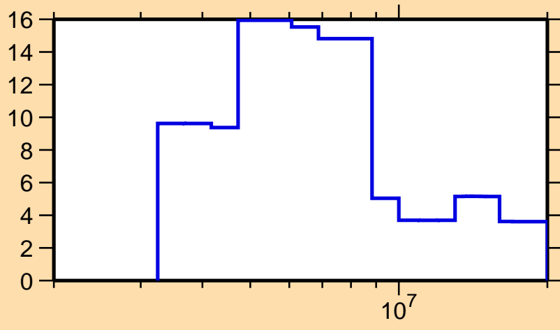
\Delta\sigma/\sigma vs. E for ^{210}\text{Au}(n,\text{tot.})
