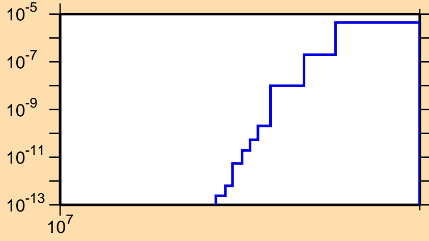
\sigma vs. E for ^{210}\text{Au}(n,\text{nd})
