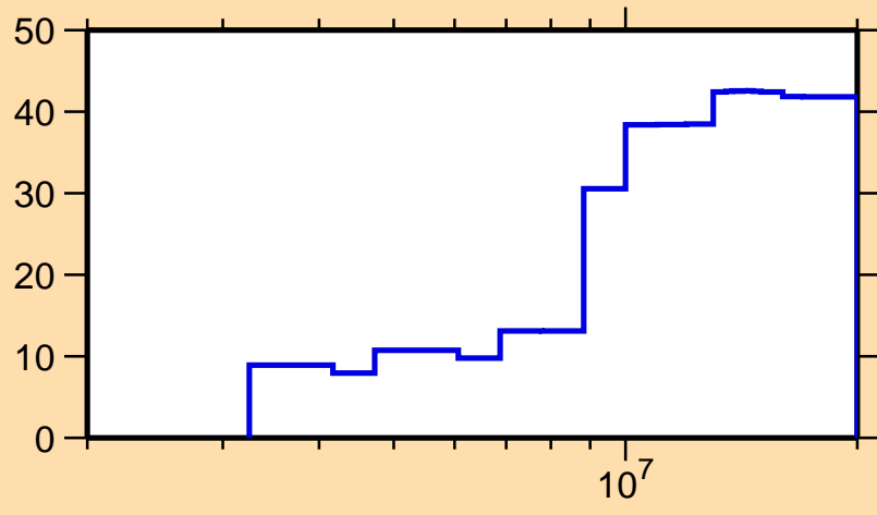
\Delta\sigma/\sigma vs. E for ^{210}\text{Au}(n,2n)
