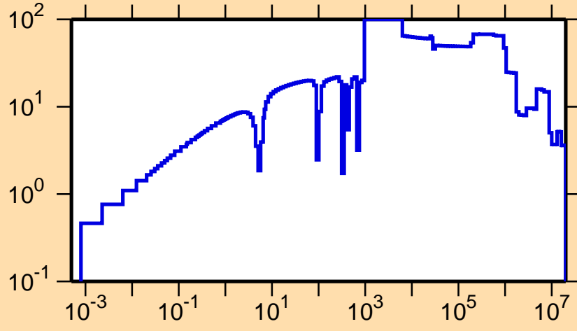
\Delta\sigma/\sigma vs. E for ^{210}\text{Au}(n,\text{tot.})
