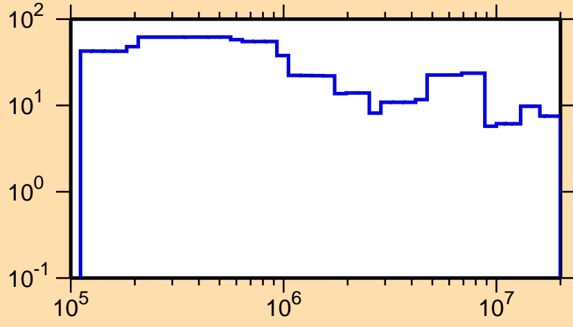
\Delta\sigma/\sigma vs. E for ^{210}\text{Au}(n,\text{el.})
