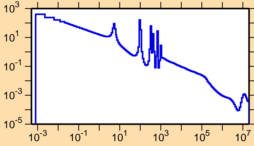
\sigma vs. E for ^{210}\text{Au}(n,\gamma)
