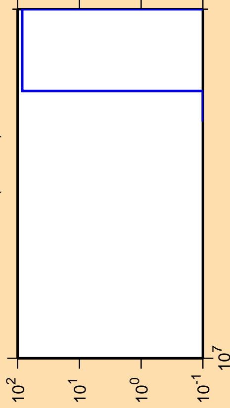
\Delta\sigma/\sigma vs. E for ^{210}\text{Au} (mt 11)
