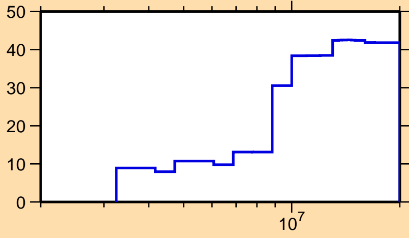
\Delta\sigma/\sigma vs. E for ^{210}\text{Au}(n,2n)
