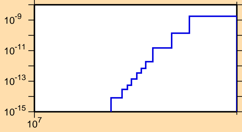
\sigma vs. E for ^{210}\text{Au}(n,3n\alpha)
