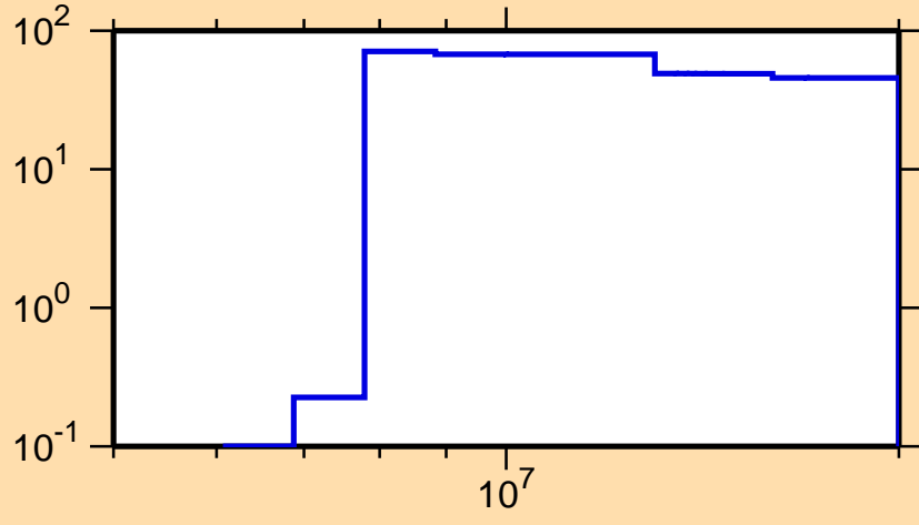
\Delta\sigma/\sigma vs. E for ^{210}\text{Au}(n,p)
