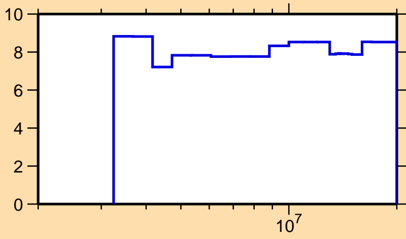
\Delta\sigma/\sigma vs. E for ^{210}\text{Au}(n,\text{nonel.})
