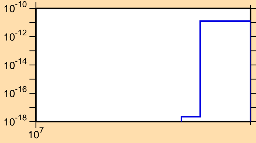
\sigma vs. E for ^{210}\text{Au} (mt 11)
