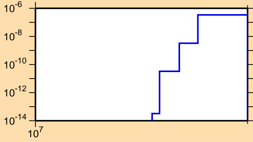
\sigma vs. E for ^{210}\text{Au}(n,2np)
