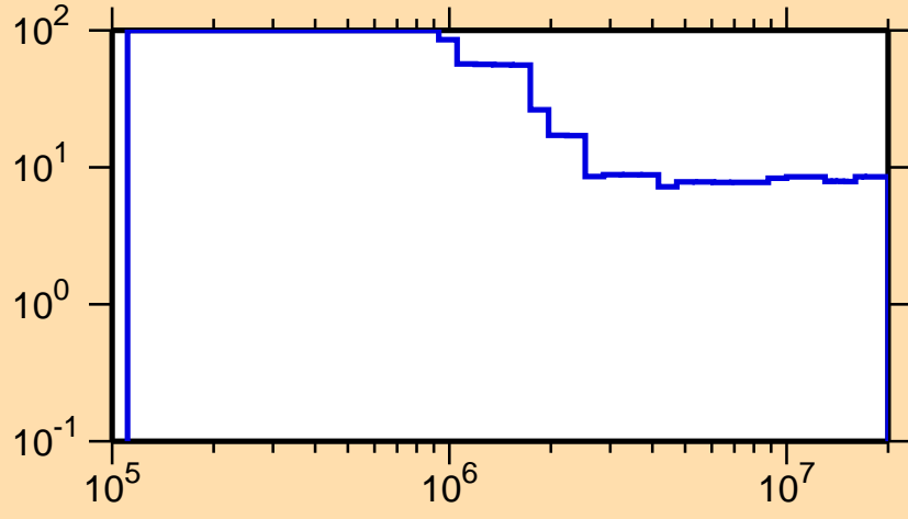
\Delta\sigma/\sigma vs. E for ^{210}\text{Au}(n,\text{nonel.})
