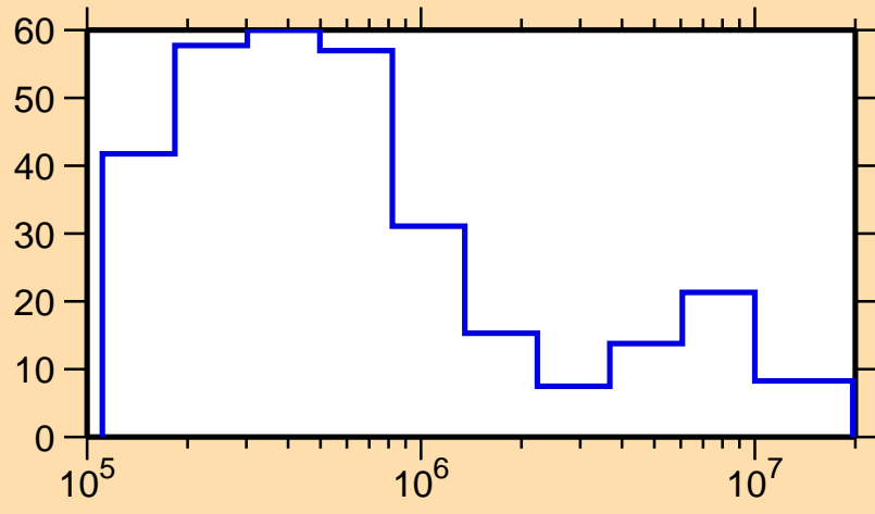
\Delta\sigma/\sigma vs. E for ^{210}\text{Au}(n,\text{el.})
