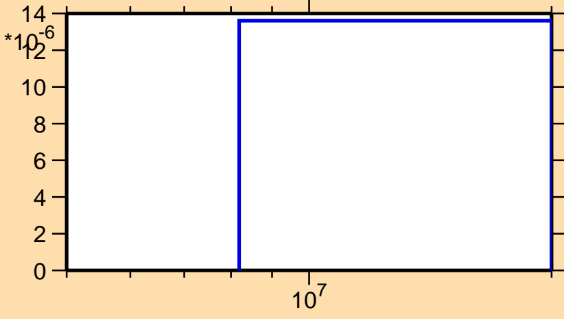
\sigma vs. E for ^{210}\text{Au}(n,t)
