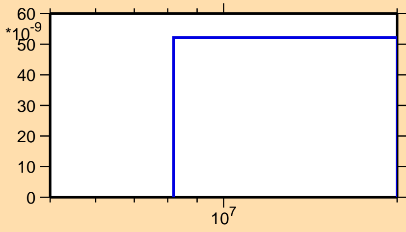
\sigma vs. E for ^{210}\text{Au}(n,2n\alpha)
