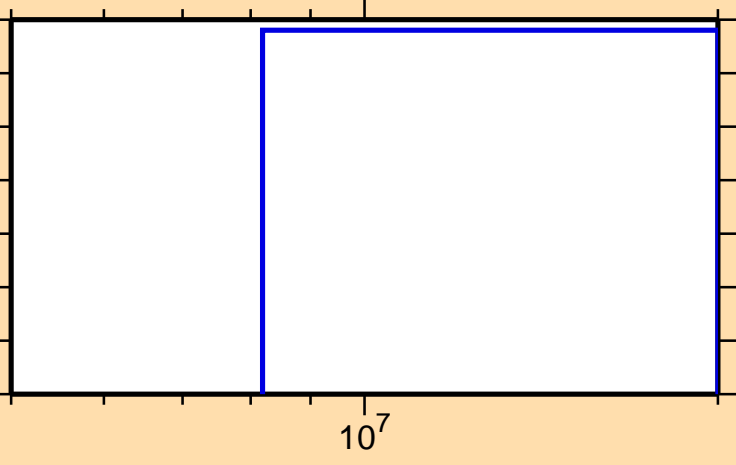
\sigma vs. E for ^{210}\text{Au}(n,t)
