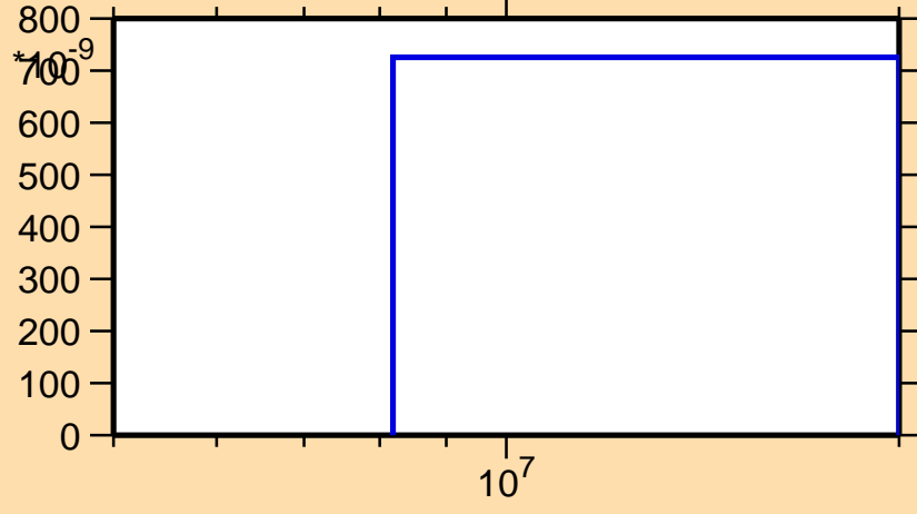
\sigma vs. E for ^{210}\text{Au}(n,nt)
