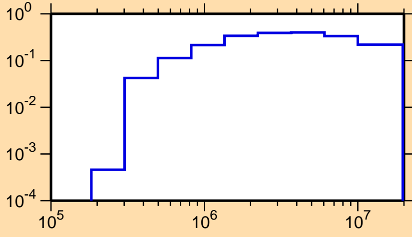
\sigma vs. E for ^{116}\text{Ba}(n,\text{inel.})
