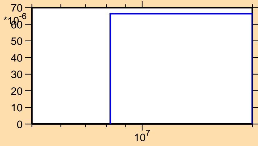
\sigma vs. E for ^{116}\text{Ba}(n,t)
