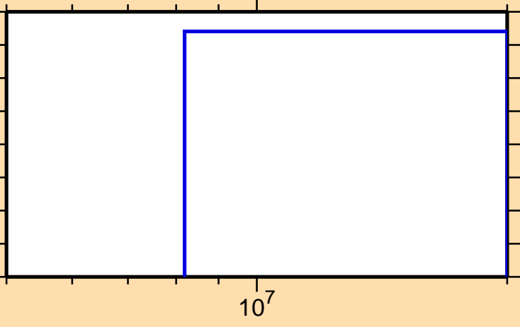
\sigma vs. E for ^{116}\text{Ba}(n,\text{pt})
