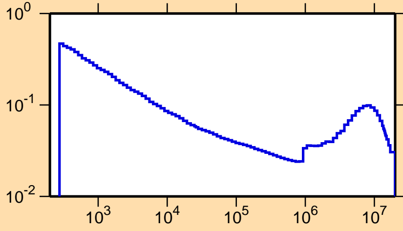
\sigma vs. E for ^{117}\text{Ba}(n,\alpha)
