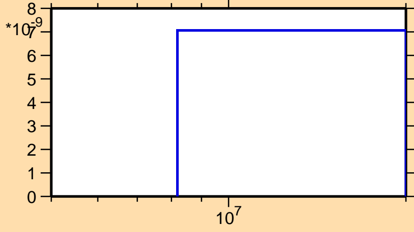
\sigma vs. E for ^{117}\text{Ba}(\text{mt } 34)
