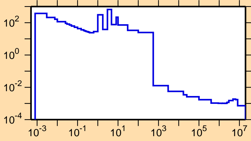
\sigma vs. E for ^{117}\text{Ba}(n,\gamma)
