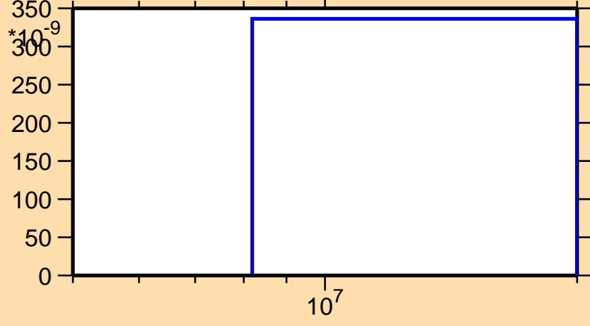
\sigma vs. E for ^{117}\text{Ba}(n,2np)
