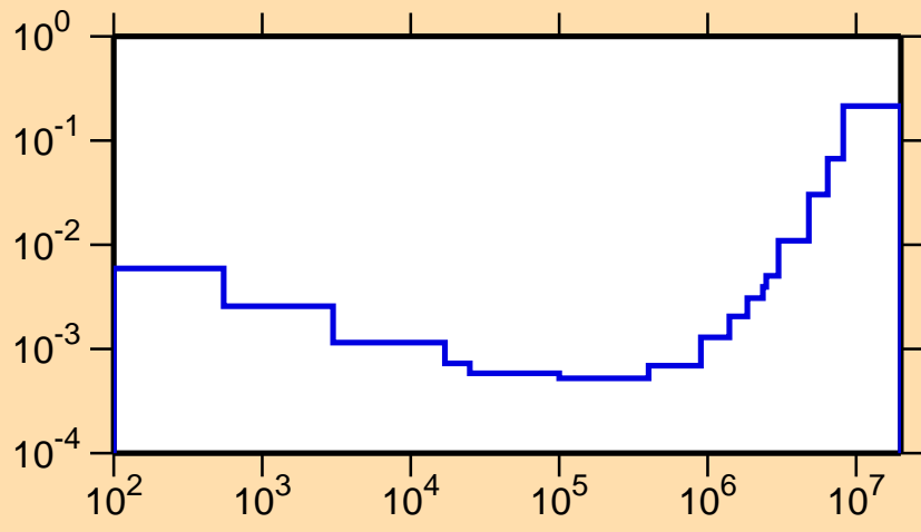
\sigma vs. E for ^{117}\text{Ba}(n,p\alpha)
