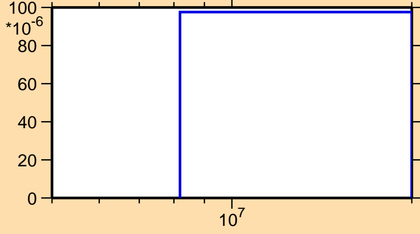
\sigma vs. E for ^{117}\text{Ba}(n,\text{pt})
