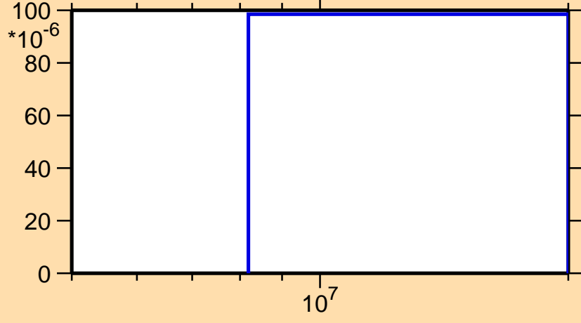
\sigma vs. E for ^{117}\text{Ba}(n,2n)
