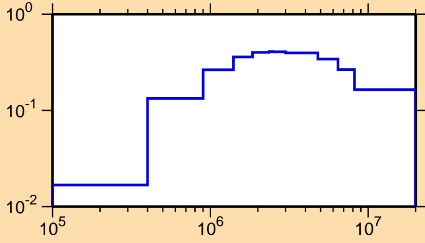
\sigma vs. E for ^{118}\text{Ba}(n,\text{inel.})
