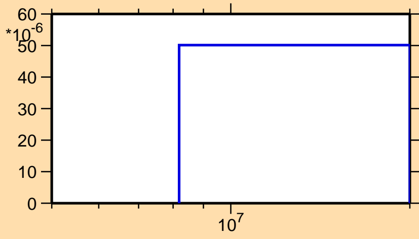
\sigma vs. E for ^{118}\text{Ba}(n,t)
