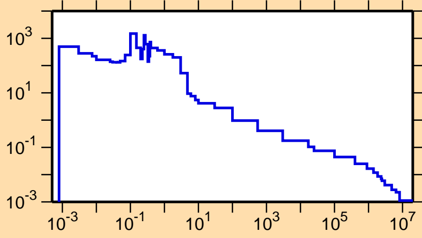
\sigma vs. E for ^{119}\text{Ba}(n,\gamma)
