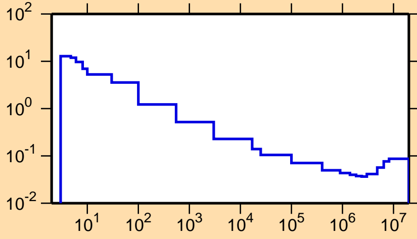
\sigma vs. E for ^{119}\text{Ba}(n,\alpha)
