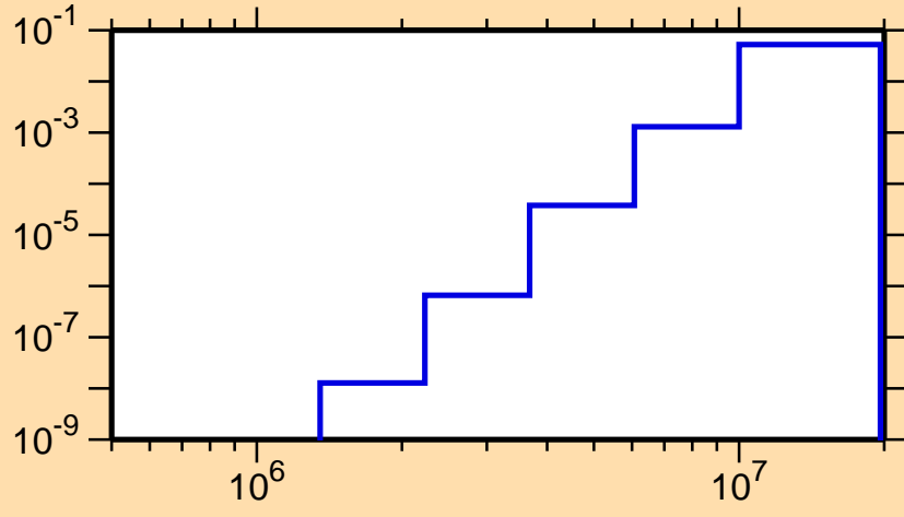
\sigma vs. E for ^{120}\text{Ba}(n,p\alpha)
