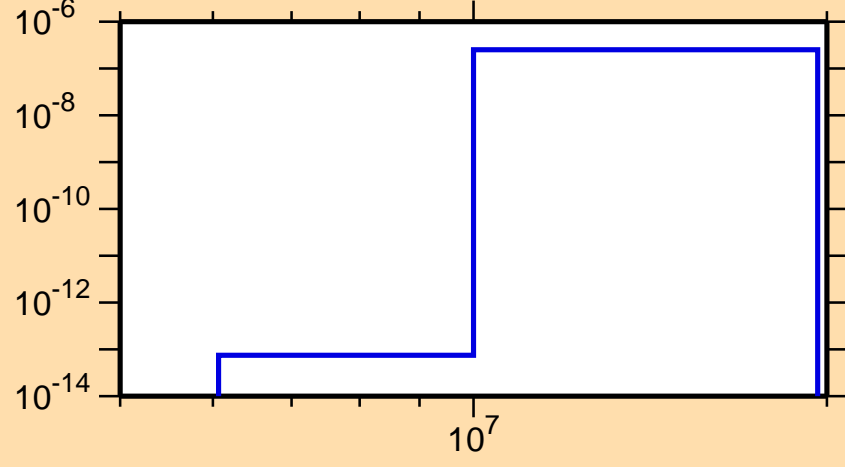
\sigma vs. E for ^{120}\text{Ba}(\text{mt117})
