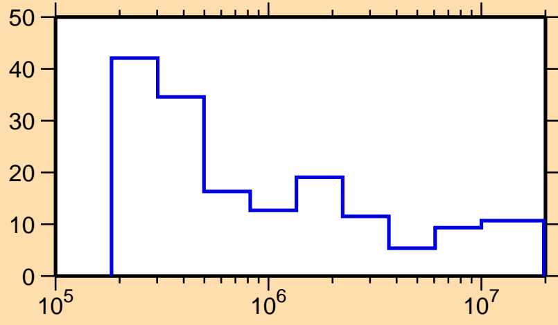
\Delta\sigma/\sigma vs. E for ^{120}\text{Ba}(n,\text{tot.})
