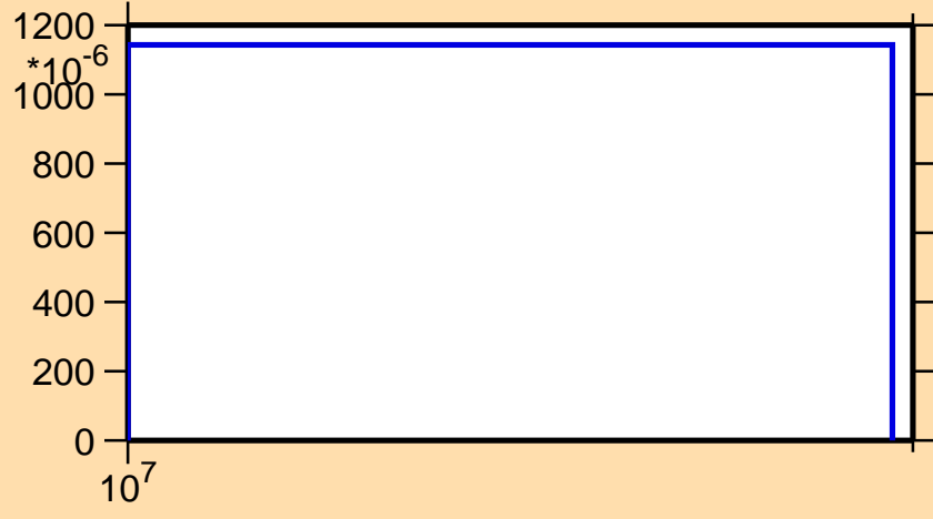
\sigma vs. E for ^{120}\text{Ba}(n,2n)
