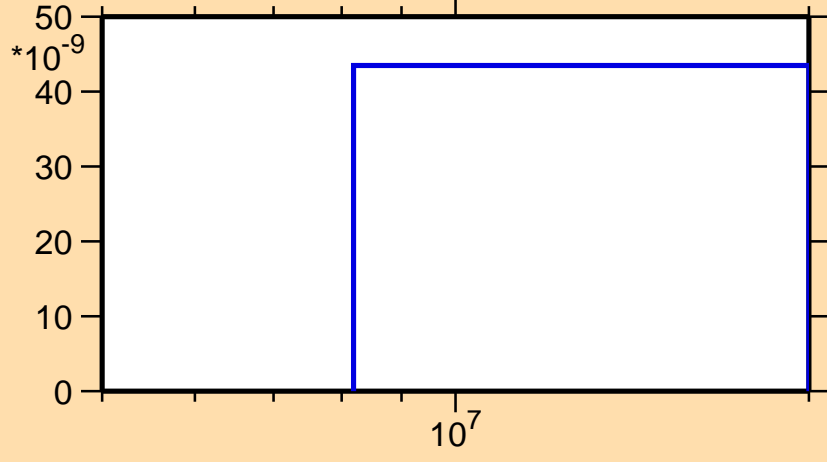
\sigma vs. E for ^{120}\text{Ba}(n,\text{pt})
