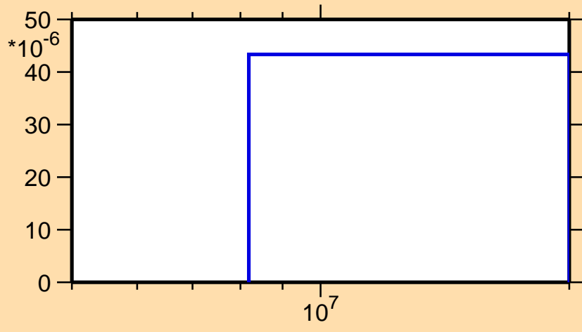
\sigma vs. E for ^{120}\text{Ba}(n,t)
