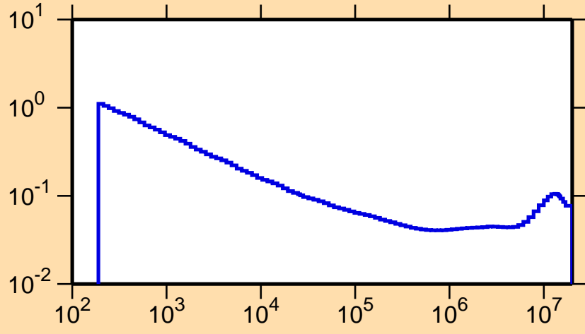
\sigma vs. E for ^{121}\text{Ba}(n,\alpha)
