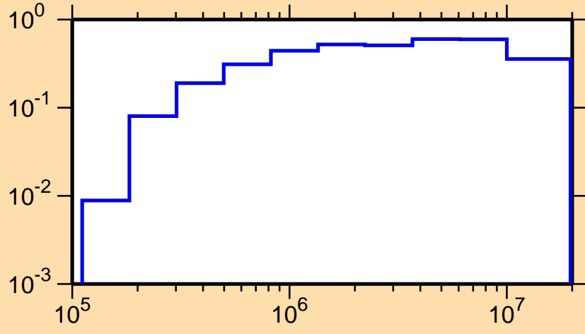
\sigma vs. E for ^{121}\text{Ba}(n,\text{inel.})
