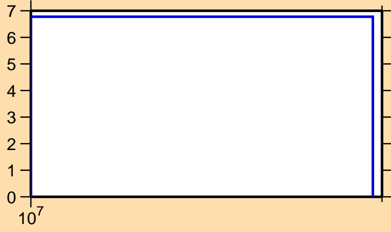
\Delta\sigma/\sigma vs. E for ^{121}\text{Ba}(n,\text{tot.})
