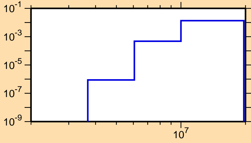
\sigma vs. E for ^{121}\text{Ba}(n,n\alpha)
