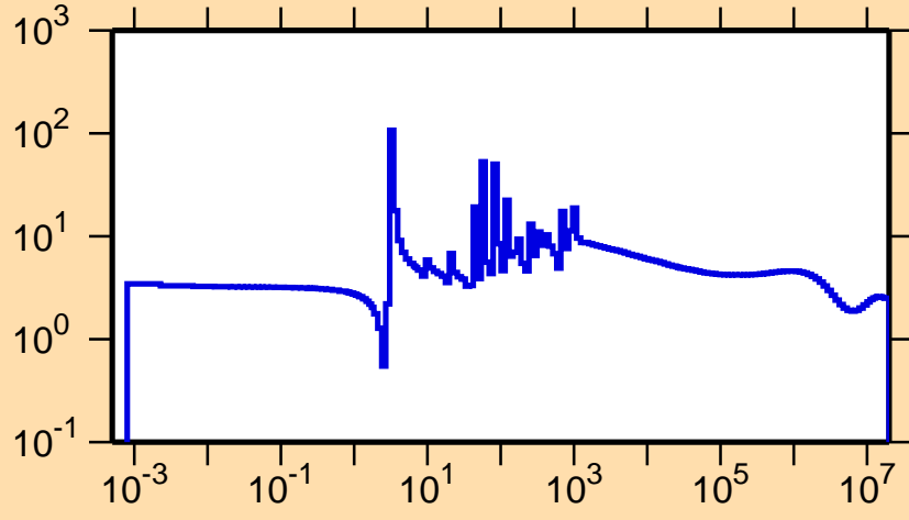
\sigma vs. E for ^{122}\text{Ba}(n,\text{el.})
