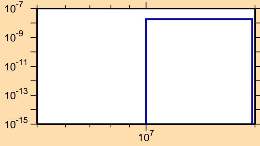
\sigma vs. E for ^{122}\text{Ba}(\text{mt117})
