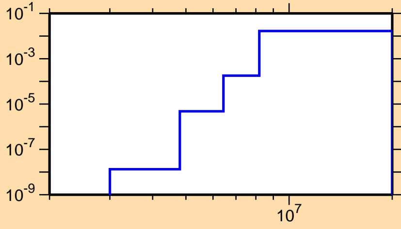
\sigma vs. E for ^{122}\text{Ba}(n,n\alpha)
