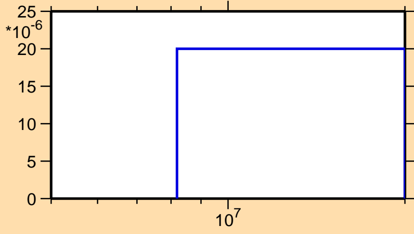
\sigma vs. E for ^{122}\text{Ba}(n,\text{pd})
