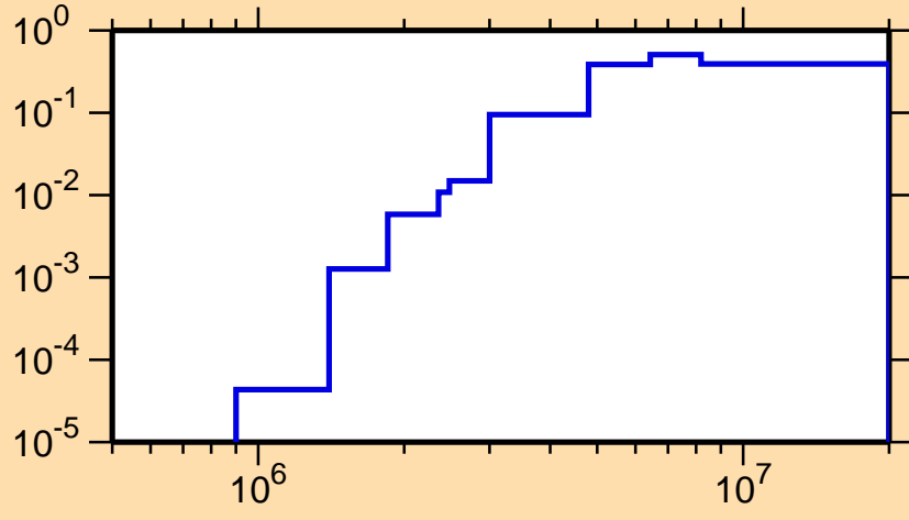
\sigma vs. E for ^{122}\text{Ba}(n,n\text{cont.})
