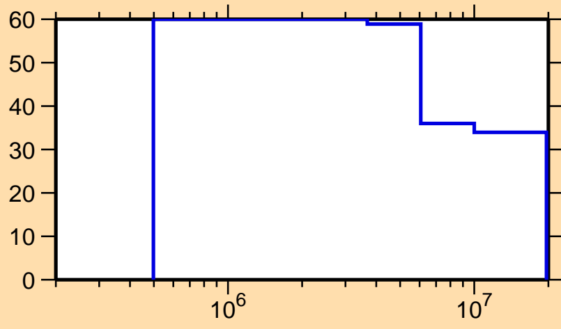
\Delta\sigma/\sigma vs. E for ^{123}\text{Ba}(n,n\text{cont.})
