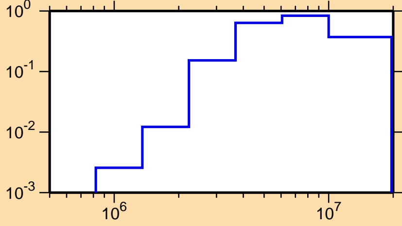
\sigma vs. E for ^{123}\text{Ba}(n,n\text{cont.})
