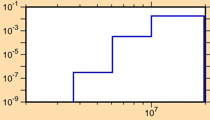
\sigma vs. E for ^{123}\text{Ba}(n,n\alpha)
