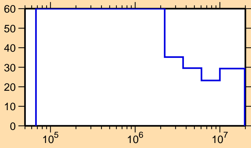
\Delta\sigma/\sigma vs. E for ^{123}\text{Ba}(n,\text{inel.})
