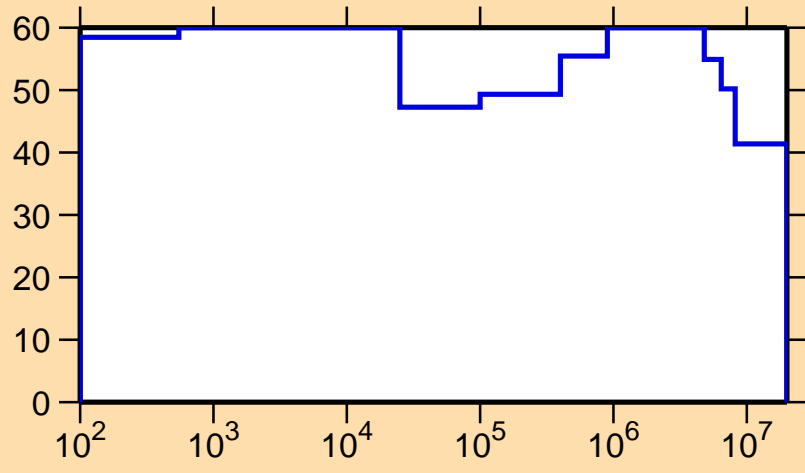
\Delta\sigma/\sigma vs. E for ^{123}\text{Ba}(n,\gamma)
