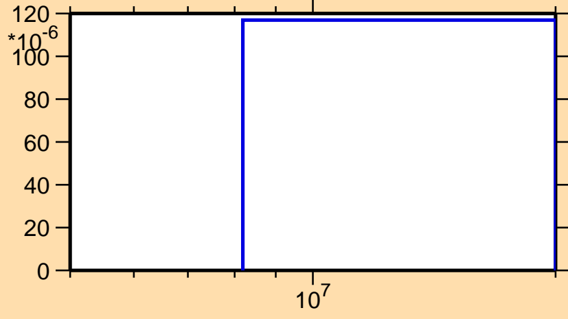
\sigma vs. E for ^{123}\text{Ba}(n,t)
