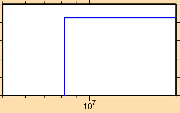
\sigma vs. E for ^{123}\text{Ba}(n,\text{nd})
