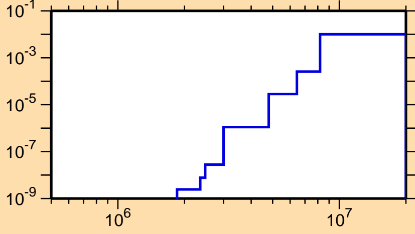
\sigma vs. E for ^{123}\text{Ba}(n,p\alpha)
