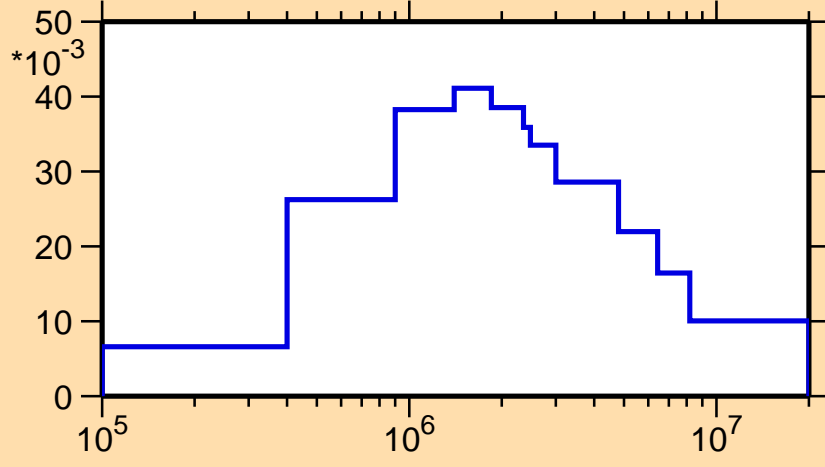
\sigma vs. E for ^{123}\text{Ba}(n,n_2)
