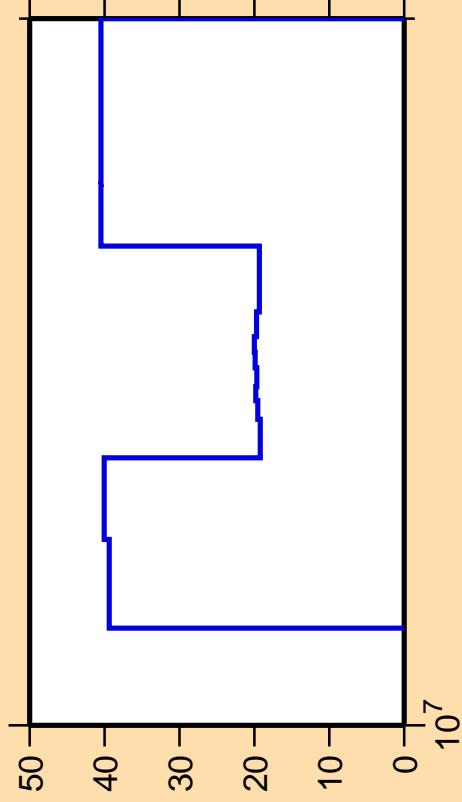
\Delta\sigma/\sigma vs. E for ^{124}\text{Ba}(n,\gamma)
