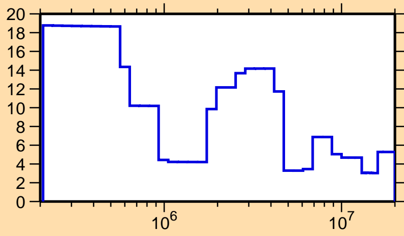
\Delta\sigma/\sigma vs. E for ^{124}\text{Ba}(n,\text{el.})
