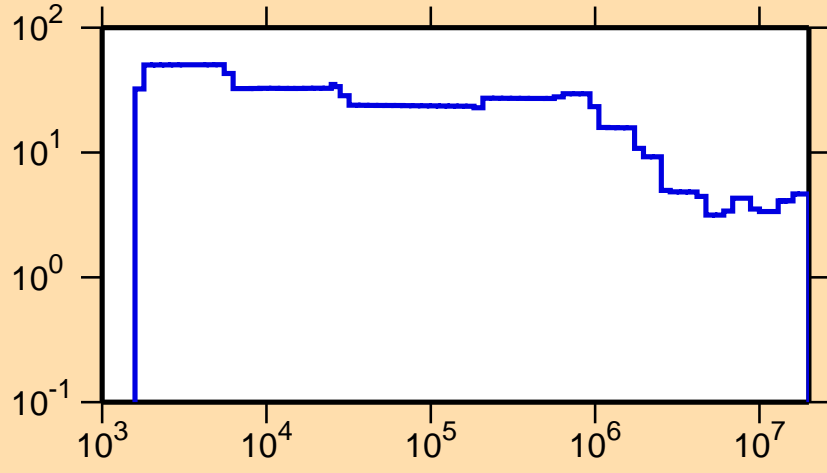
\Delta\sigma/\sigma vs. E for ^{124}\text{Ba}(n,\text{nonel.})
