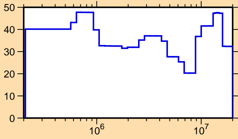
\Delta\sigma/\sigma vs. E for ^{124}\text{Ba}(n,\text{inel.})
