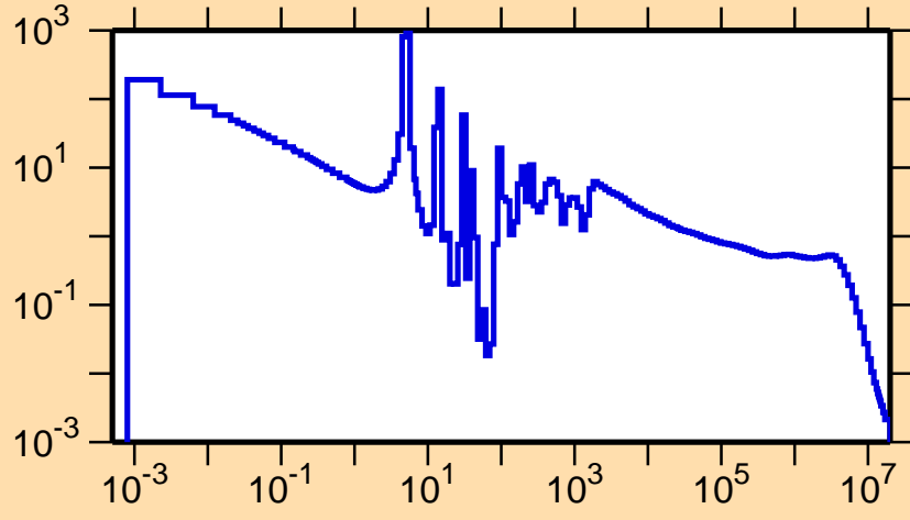
\sigma vs. E for ^{124}\text{Ba}(n,\gamma)
