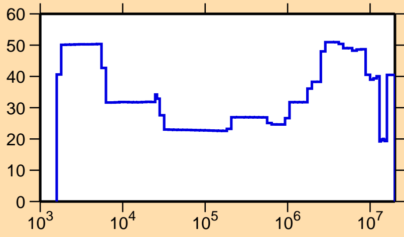
\Delta\sigma/\sigma vs. E for ^{124}\text{Ba}(n,\gamma)
