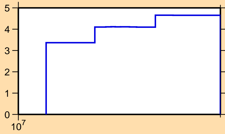
\Delta\sigma/\sigma vs. E for ^{124}\text{Ba}(n,\text{nonel.})
