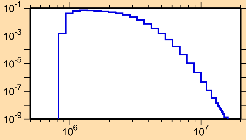
\sigma vs. E for ^{124}\text{Ba}(n,n_4)
