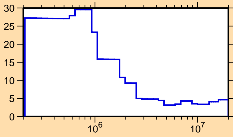
\Delta\sigma/\sigma vs. E for ^{124}\text{Ba}(n,\text{nonel.})
