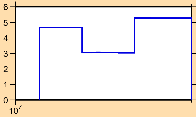
\Delta\sigma/\sigma vs. E for ^{124}\text{Ba}(n,\text{el.})
