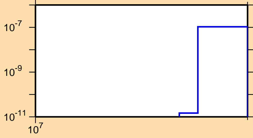
\sigma vs. E for ^{124}\text{Ba}(n,\text{nd})
