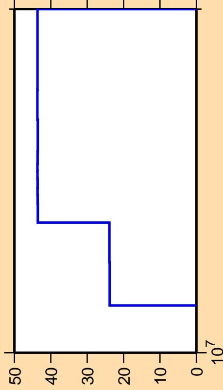
\Delta\sigma/\sigma vs. E for ^{124}\text{Ba}(n,p)
