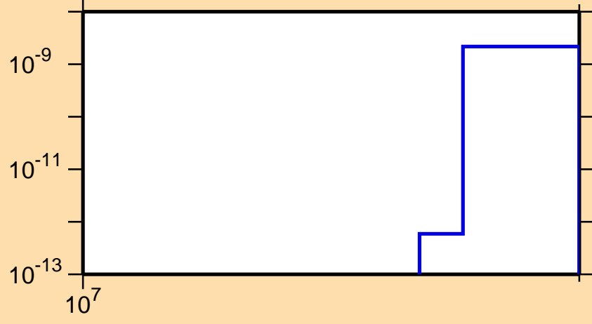
\sigma vs. E for ^{124}\text{Ba}(n,\text{pt})
