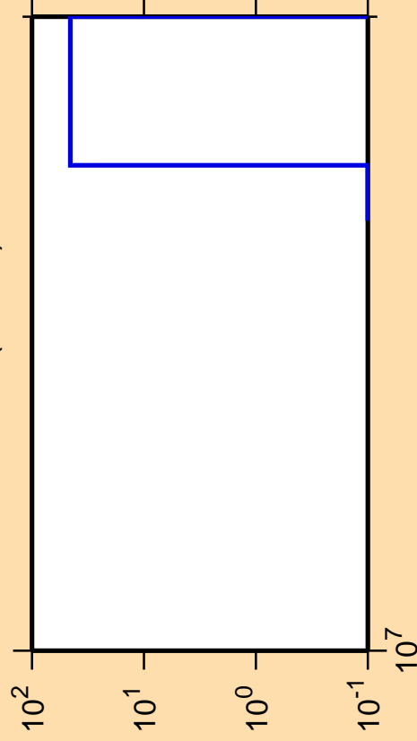
\Delta\sigma/\sigma vs. E for ^{124}\text{Ba} (mt 34)
