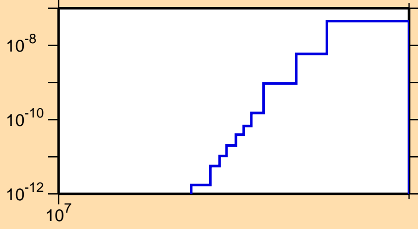
\sigma vs. E for ^{124}\text{Ba}(\text{mt117})
