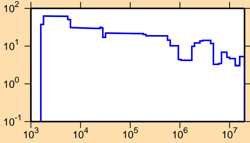
\Delta\sigma/\sigma vs. E for ^{124}\text{Ba}(n,\text{el.})
