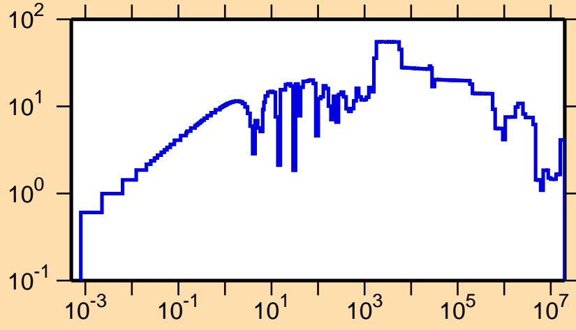
\Delta\sigma/\sigma vs. E for ^{124}\text{Ba}(n,\text{tot.})
