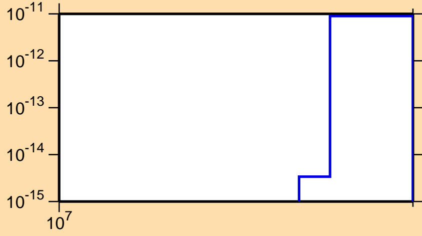
\sigma vs. E for ^{124}\text{Ba} (mt 34)
