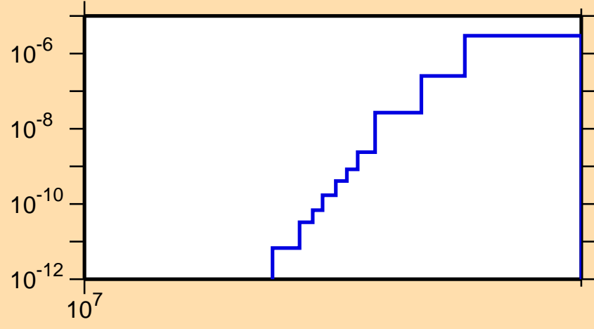
\sigma vs. E for ^{124}\text{Ba} (mt 45)
