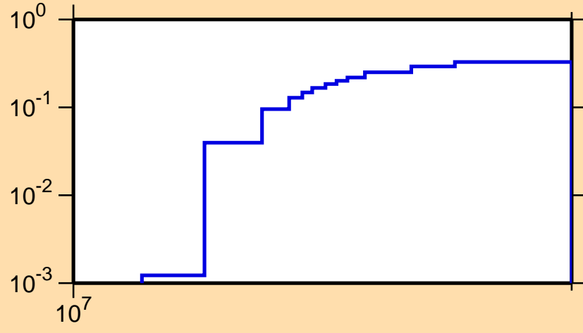
\sigma vs. E for ^{124}\text{Ba}(n,2n)
