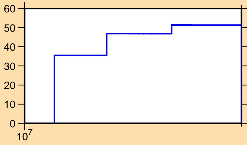
\Delta\sigma/\sigma vs. E for ^{124}\text{Ba}(n,2n)
