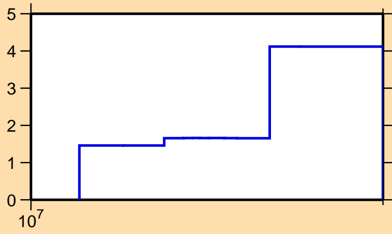
\Delta\sigma/\sigma vs. E for ^{124}\text{Ba}(n,\text{tot.})
