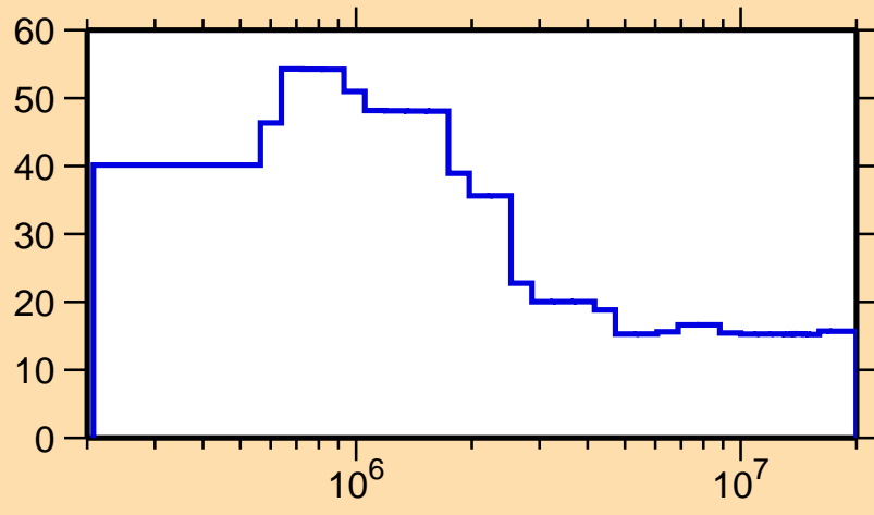
\Delta\sigma/\sigma vs. E for ^{124}\text{Ba}(n,n_1)
