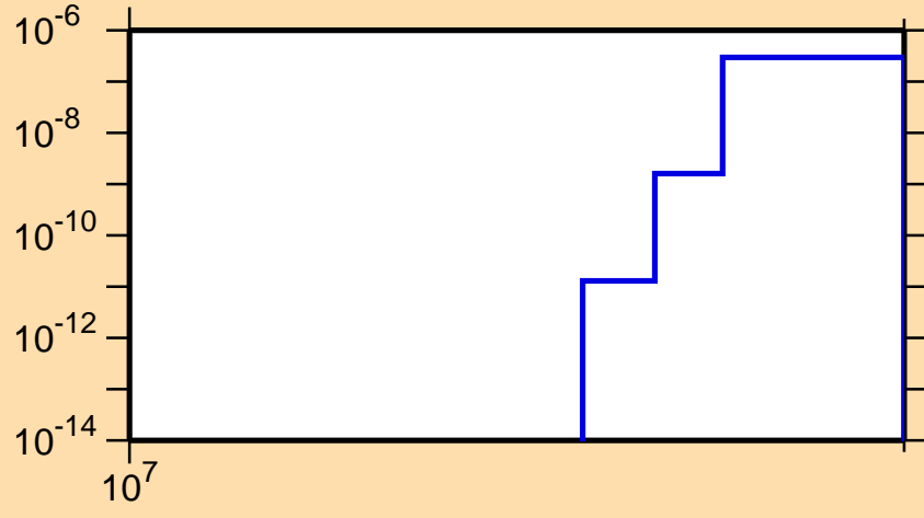
\sigma vs. E for ^{124}\text{Ba}(n,2n\alpha)
