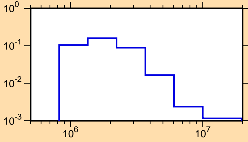
\sigma vs. E for ^{124}\text{Ba}(n,n_3)
