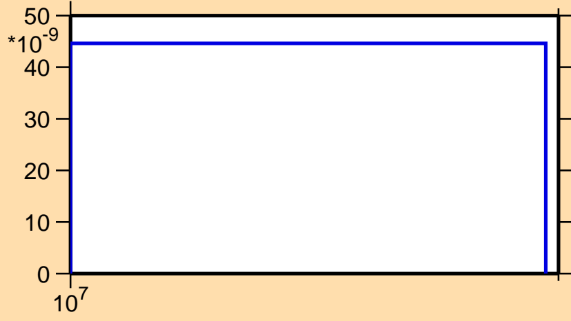
\sigma vs. E for ^{124}\text{Ba} (mt 45)
