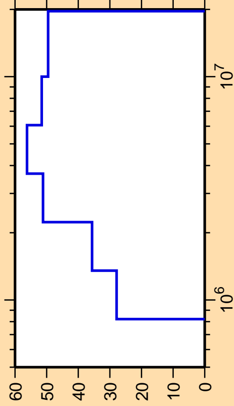
\Delta\sigma/\sigma vs. E for ^{124}\text{Ba}(n,n_4)
