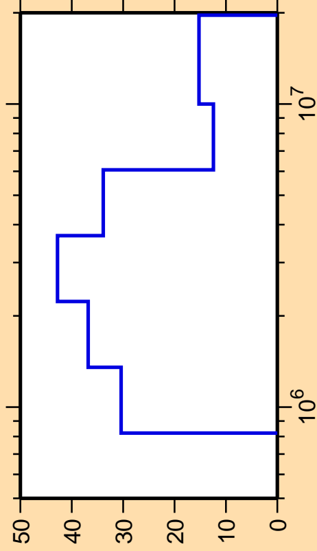
\Delta\sigma/\sigma vs. E for ^{124}\text{Ba}(n,n_3)
