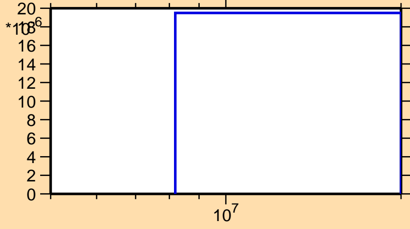
\sigma vs. E for ^{124}\text{Ba}(n,t)
