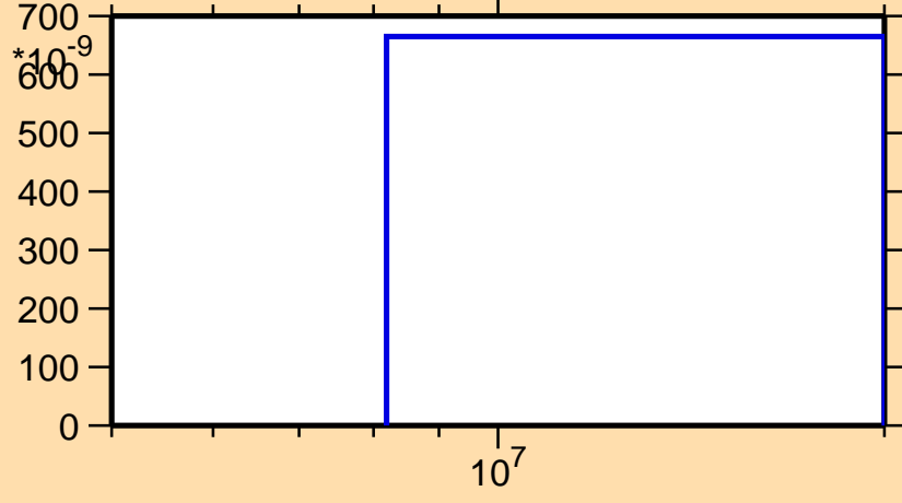
\sigma vs. E for ^{124}\text{Ba}(n,\text{pd})
