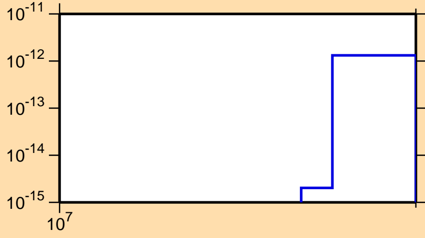
\sigma vs. E for ^{125}\text{Ba}(n,nt)
