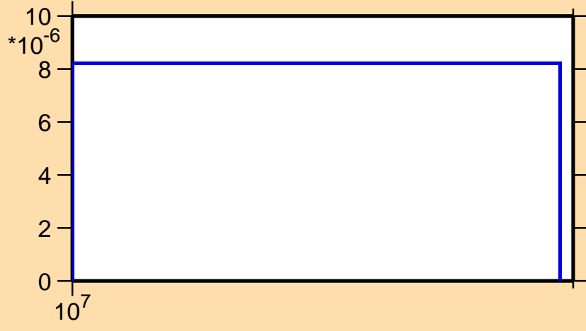
\sigma vs. E for ^{125}\text{Ba}(n,2np)
