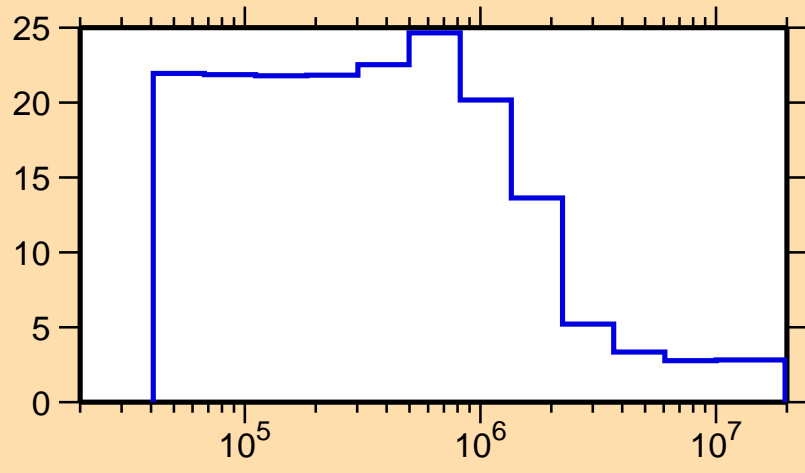
\Delta\sigma/\sigma vs. E for ^{125}\text{Ba}(n,\text{nonel.})
