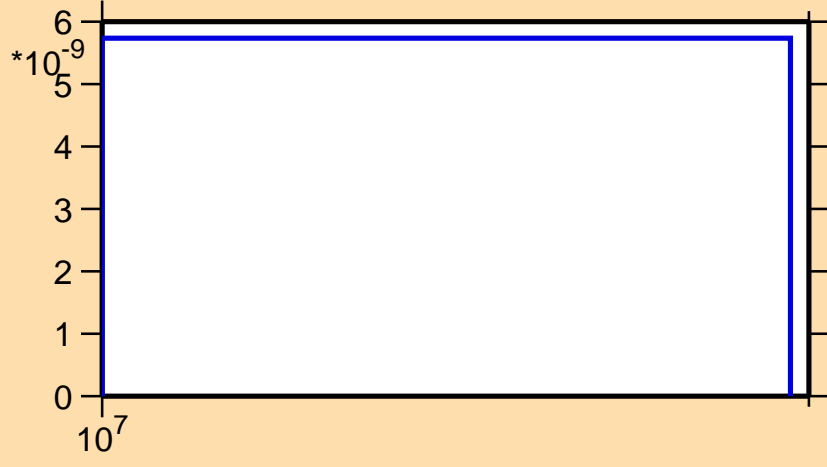
\sigma vs. E for ^{125}\text{Ba}(n,\text{pt})
