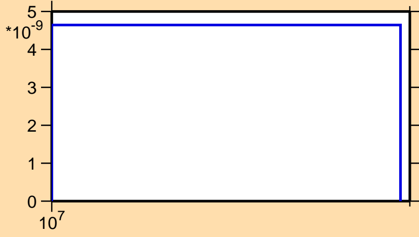
\sigma vs. E for ^{126}\text{Ba}(n,2n\alpha)
