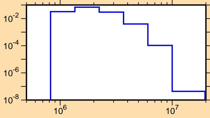
\sigma vs. E for ^{126}\text{Ba}(n,n_4)
