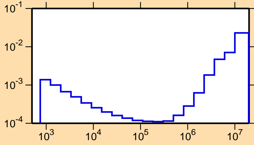
\sigma vs. E for ^{126}\text{Ba}(n,\alpha)
