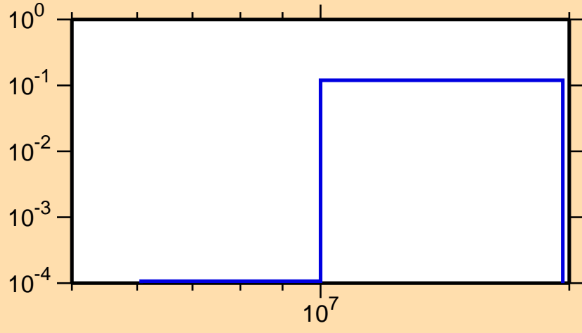
\sigma vs. E for ^{126}\text{Ba}(n,np)
