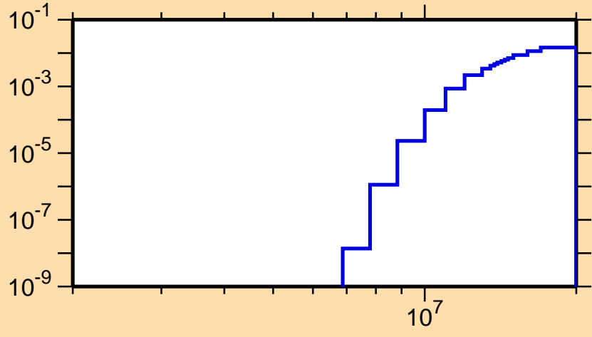
\sigma vs. E for ^{127}\text{Ba}(n,d)
