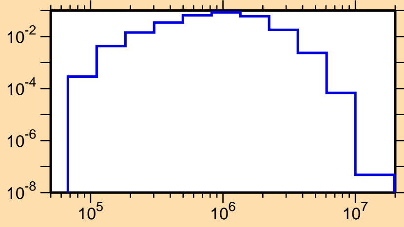
\sigma vs. E for ^{127}\text{Ba}(n,n_2)
