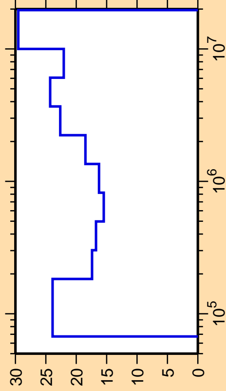
\Delta\sigma/\sigma vs. E for ^{127}\text{Ba}(n,n_2)
