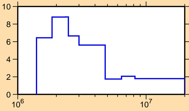
\Delta\sigma/\sigma vs. E for ^{127}\text{Ba}(n, tot.)
