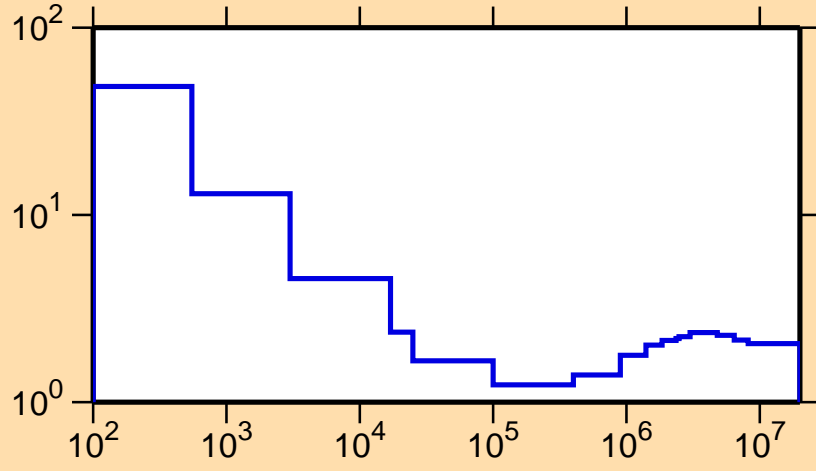
\sigma vs. E for ^{127}\text{Ba}(n,\text{nonel.})
