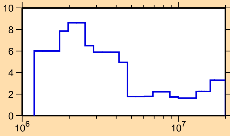
\Delta\sigma/\sigma vs. E for ^{127}\text{Ba}(n,\text{tot.})
