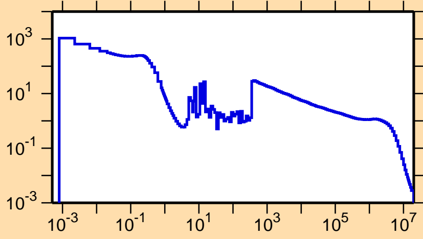
\sigma vs. E for ^{127}\text{Ba}(n,\gamma)
