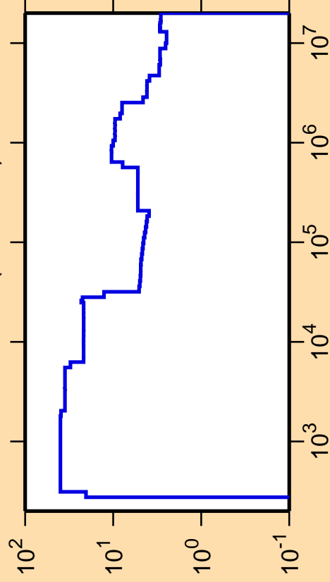
\Delta\sigma/\sigma vs. E for ^{127}\text{Ba}(n,\text{nonel.})
