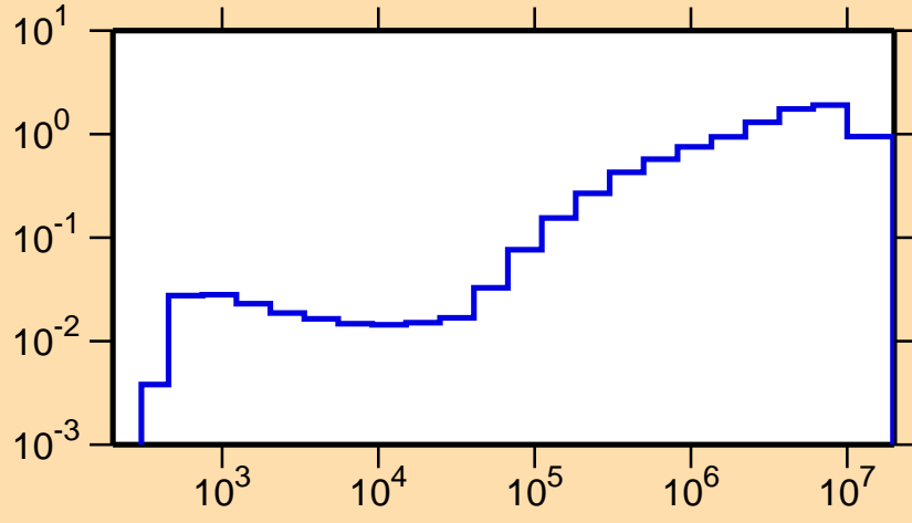
\sigma vs. E for ^{127}\text{Ba}(n,\text{inel.})
