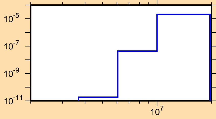
\sigma vs. E for ^{127}\text{Ba}(n,p\alpha)
