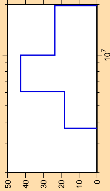
\Delta\sigma/\sigma vs. E for ^{127}\text{Ba}(n,p\alpha)
