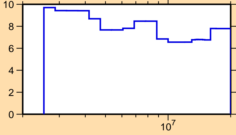
\Delta\sigma/\sigma vs. E for ^{128}\text{Ba}(n,\text{nonel.})
