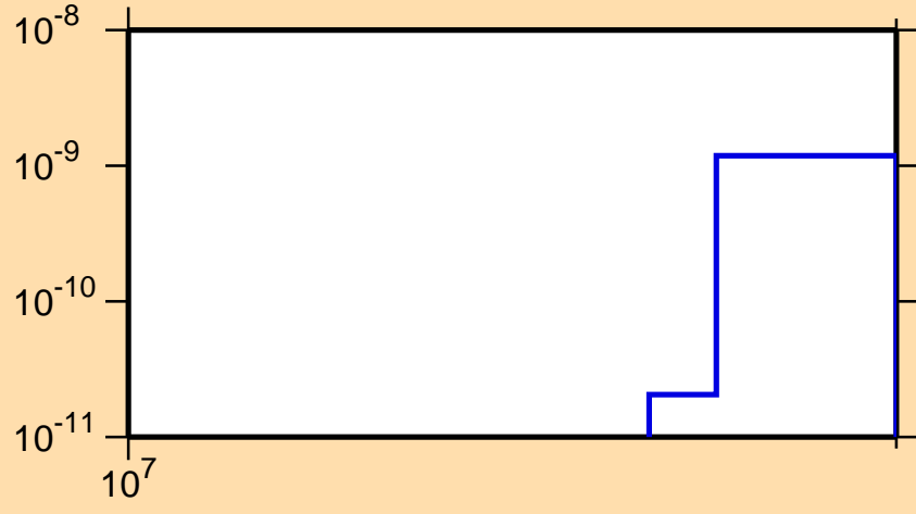
\sigma vs. E for ^{128}\text{Ba} (mt 45)
