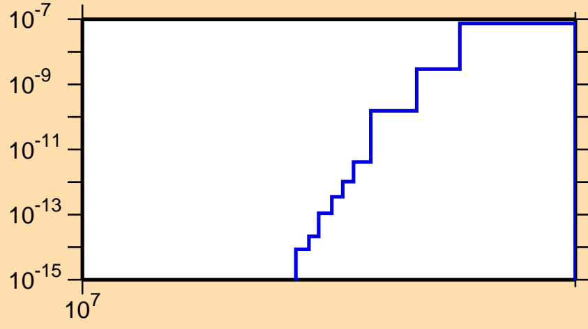
\sigma vs. E for ^{128}\text{Ba}(n,\text{pd})
