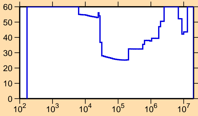
\Delta\sigma/\sigma vs. E for ^{128}\text{Ba}(n,p)
