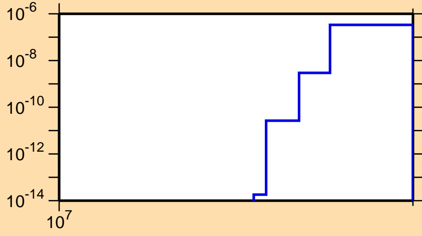
\sigma vs. E for ^{128}\text{Ba}(n,2n\alpha)
