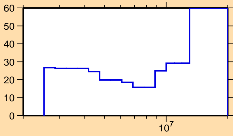
\Delta\sigma/\sigma vs. E for ^{128}\text{Ba}(n,n\text{cont.})
