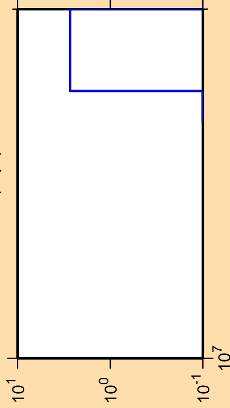
\Delta\sigma/\sigma vs. E for ^{128}\text{Ba}(n,\text{pt})
