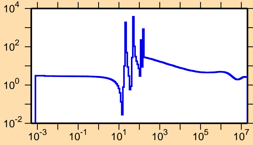
\sigma vs. E for ^{128}\text{Ba}(n,\text{el.})
