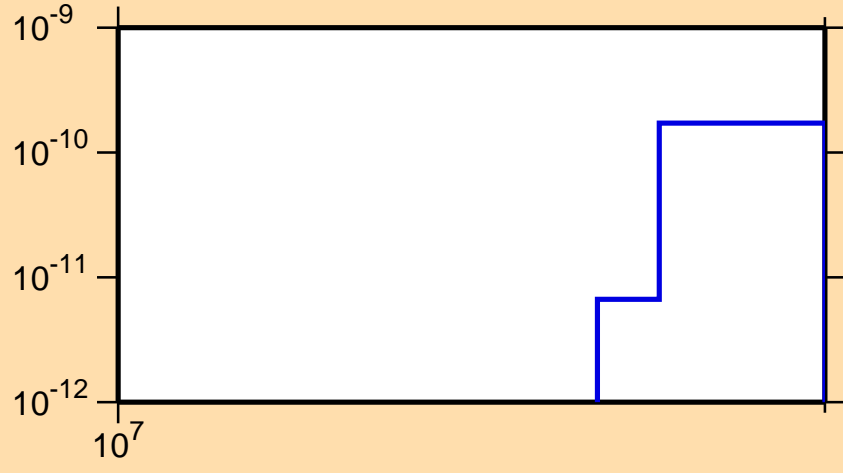
\sigma vs. E for ^{128}\text{Ba}(\text{mt117})
