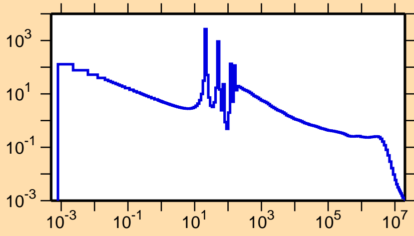
\sigma vs. E for ^{128}\text{Ba}(n,\gamma)
