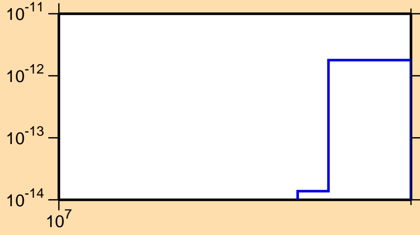
\sigma vs. E for ^{128}\text{Ba}(n,nt)
