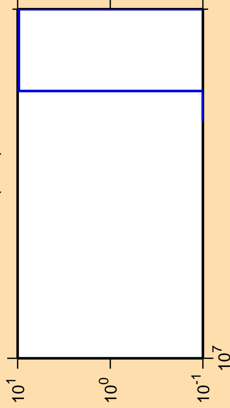
\Delta\sigma/\sigma vs. E for ^{128}\text{Ba}(n,nt)
