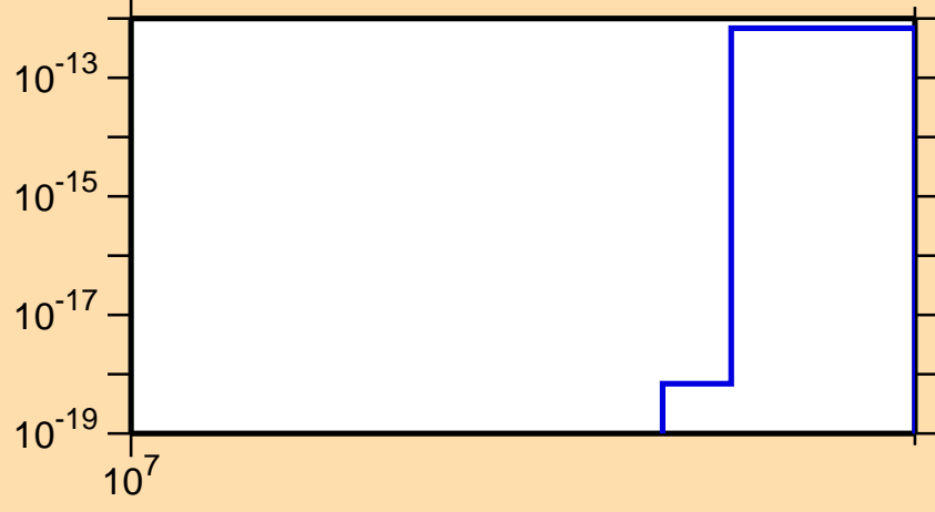
\sigma vs. E for ^{128}\text{Ba}(n,\text{pt})
