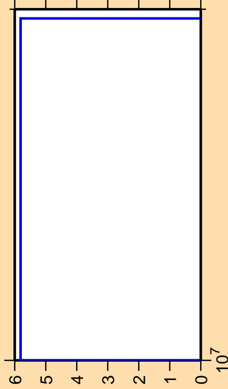
\Delta\sigma/\sigma vs. E for ^{128}\text{Ba}(\text{mt117})
