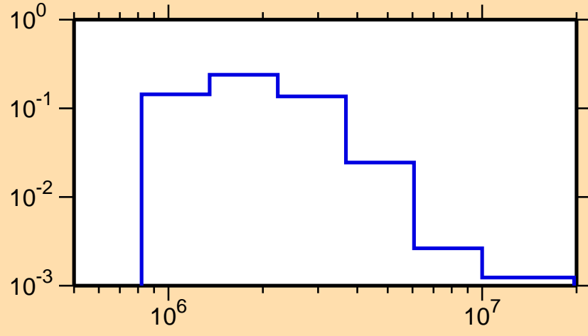
\sigma vs. E for ^{128}\text{Ba}(n,n_3)
