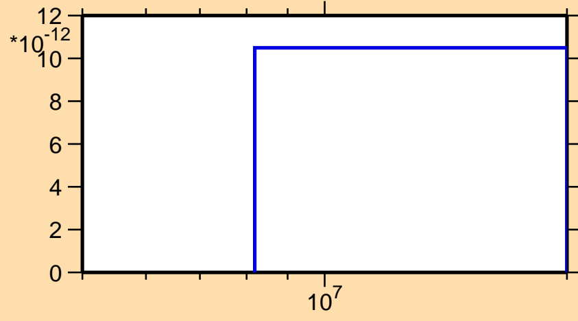
\sigma vs. E for ^{128}\text{Ba}(\text{mt } 45)
