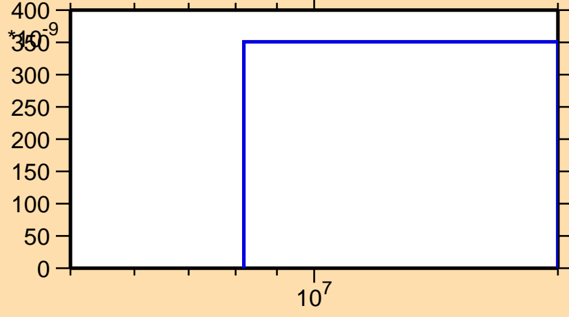
\sigma vs. E for ^{128}\text{Ba}(n,3n)
