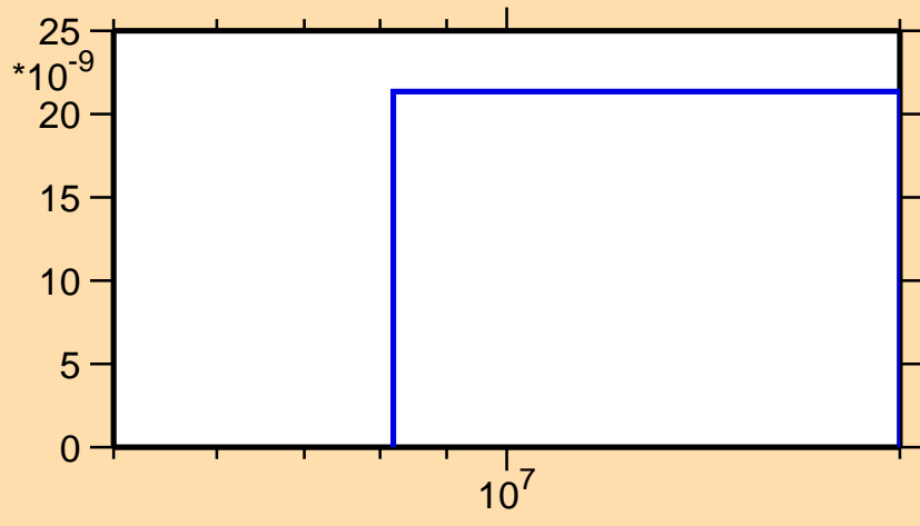
\sigma vs. E for ^{128}\text{Ba}(n,\text{He}3)
