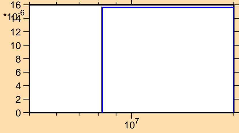
\sigma vs. E for ^{128}\text{Ba}(n,t)
