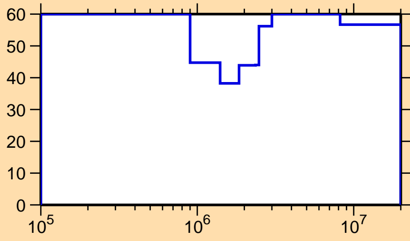
\Delta\sigma/\sigma vs. E for ^{128}\text{Ba}(n,n_1)
