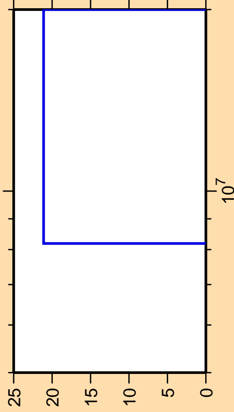
\Delta\sigma/\sigma vs. E for ^{128}\text{Ba}(\text{mt } 45)
