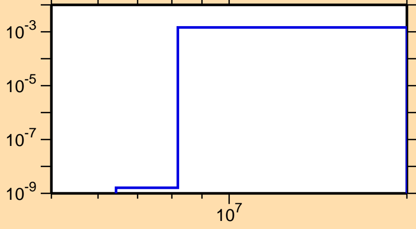
\sigma vs. E for ^{128}\text{Ba}(n,d)
