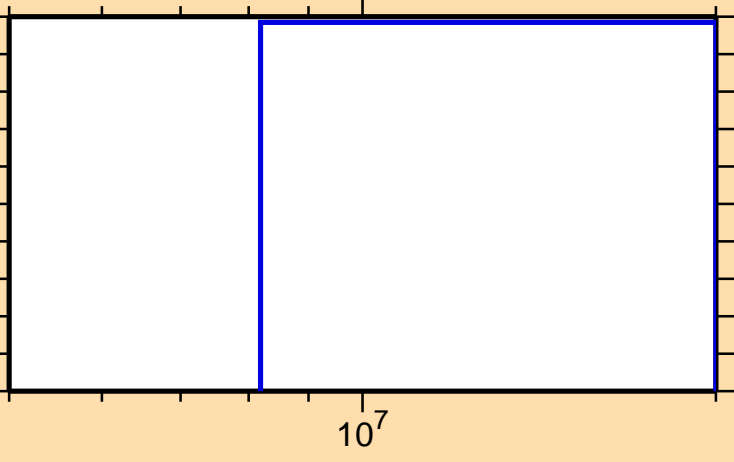
\sigma vs. E for ^{129}\text{Ba} (mt 34)
