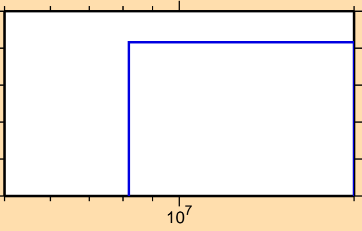
\sigma vs. E for ^{129}\text{Ba}(n,\text{He}3)
