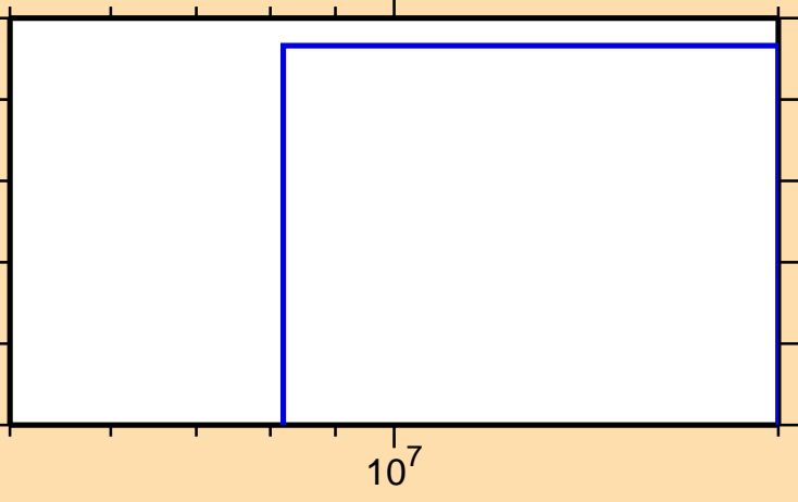
\sigma vs. E for ^{129}\text{Ba}(n,\text{nd})
