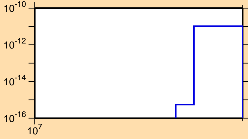
\sigma vs. E for ^{129}\text{Ba}(n,nt)
