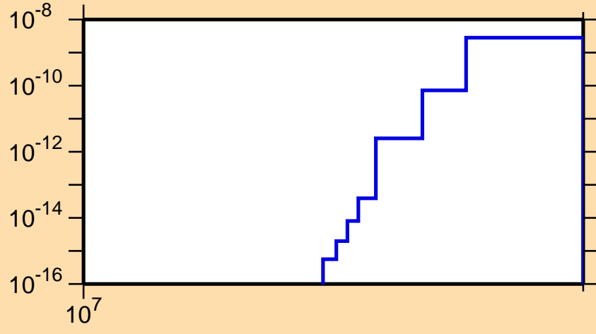
\sigma vs. E for ^{129}\text{Ba}(n,\text{pd})
