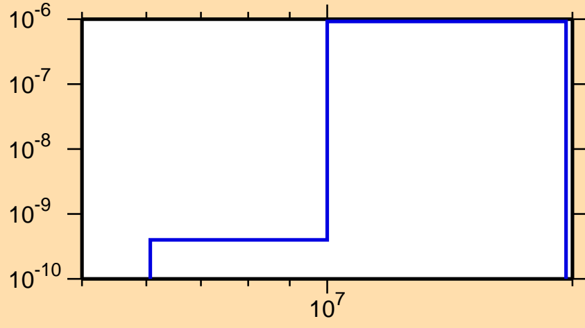
\sigma vs. E for ^{129}\text{Ba}(n,p\alpha)
