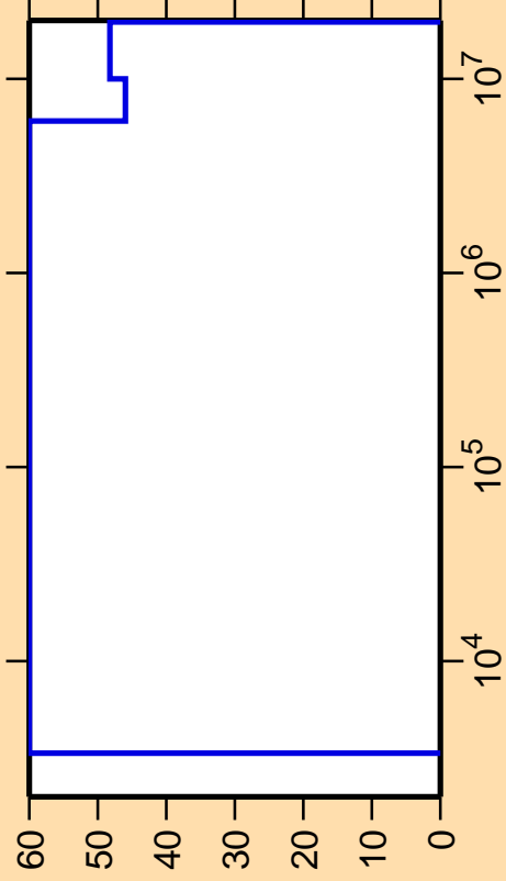
\Delta\sigma/\sigma vs. E for ^{130}\text{Ba}(n,\alpha)
