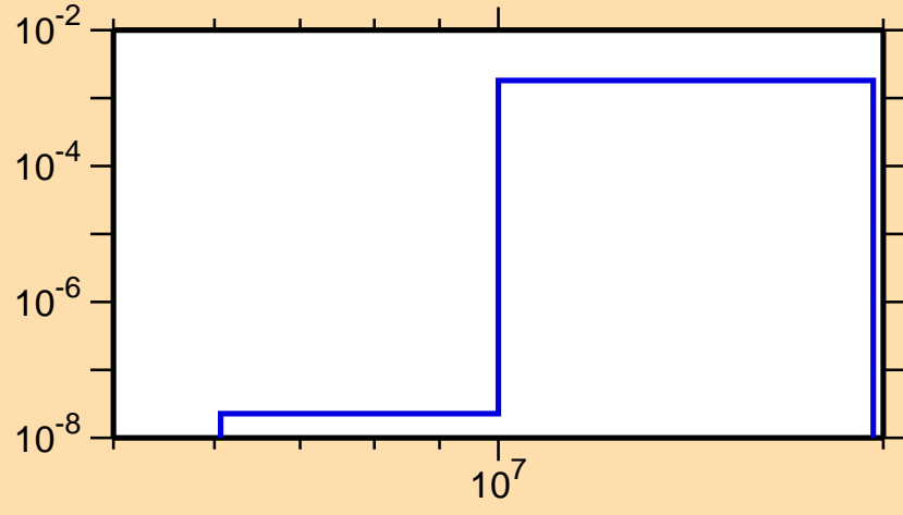
\sigma vs. E for ^{130}\text{Ba}(n,d)
