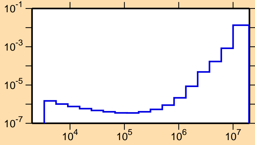
\sigma vs. E for ^{130}\text{Ba}(n,\alpha)
