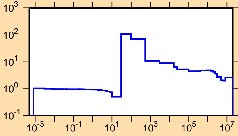
\sigma vs. E for ^{130}\text{Ba}(n,\text{el.})
