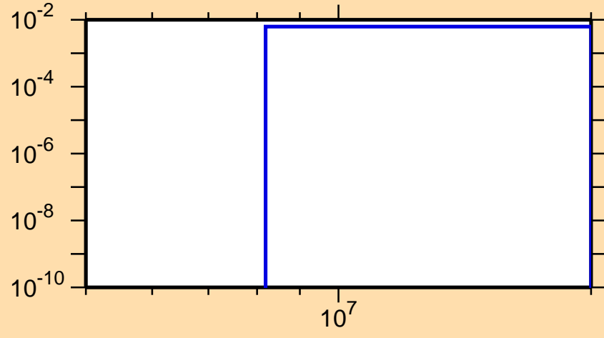
\sigma vs. E for ^{130}\text{Ba}(n,np)
