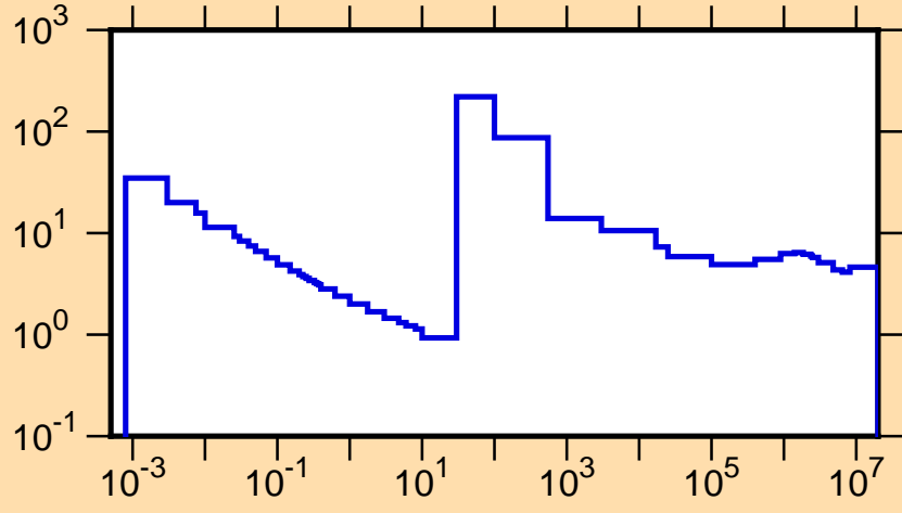
\sigma vs. E for ^{130}\text{Ba}(n,\text{tot.})
